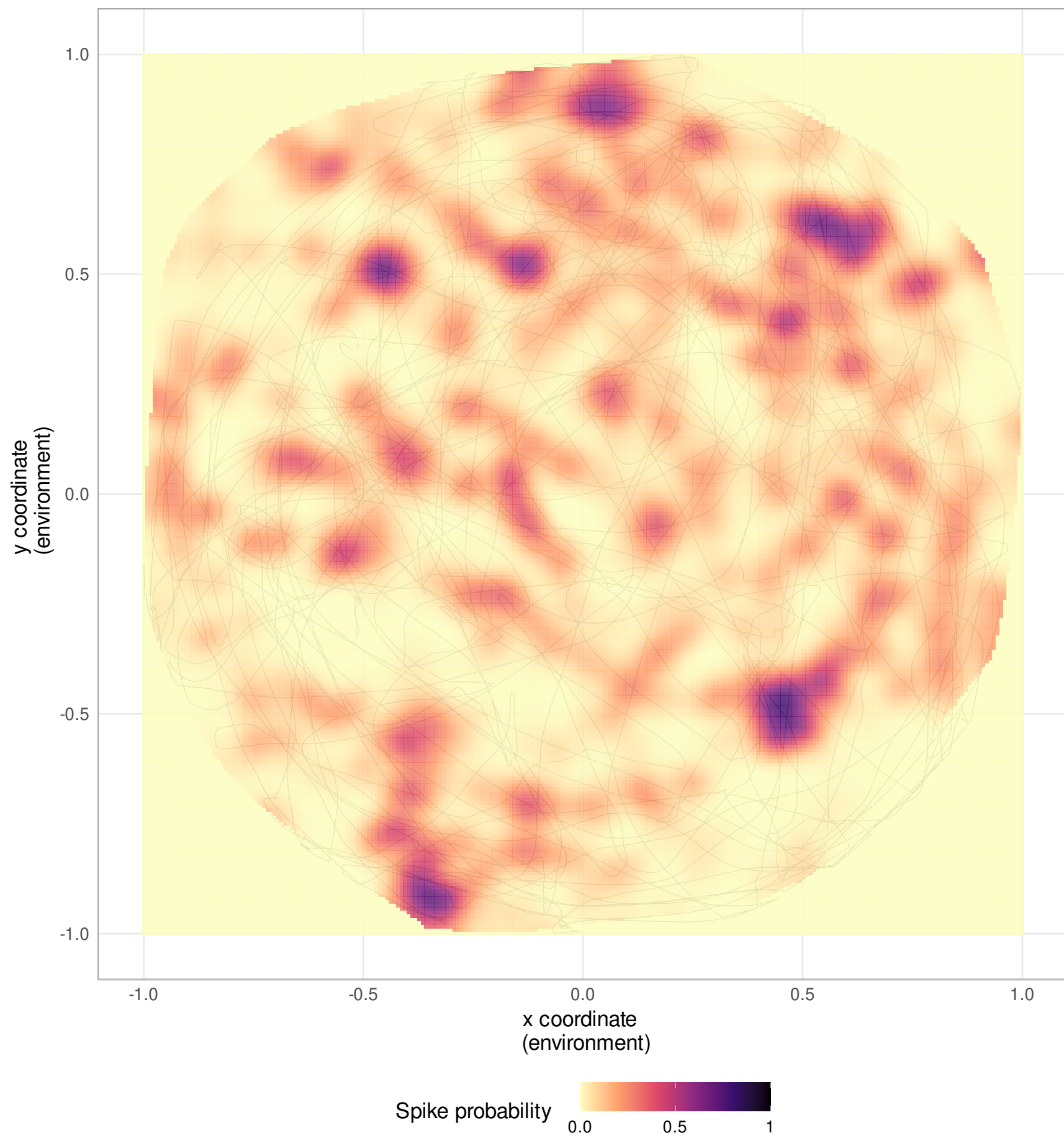
Neuron 65
