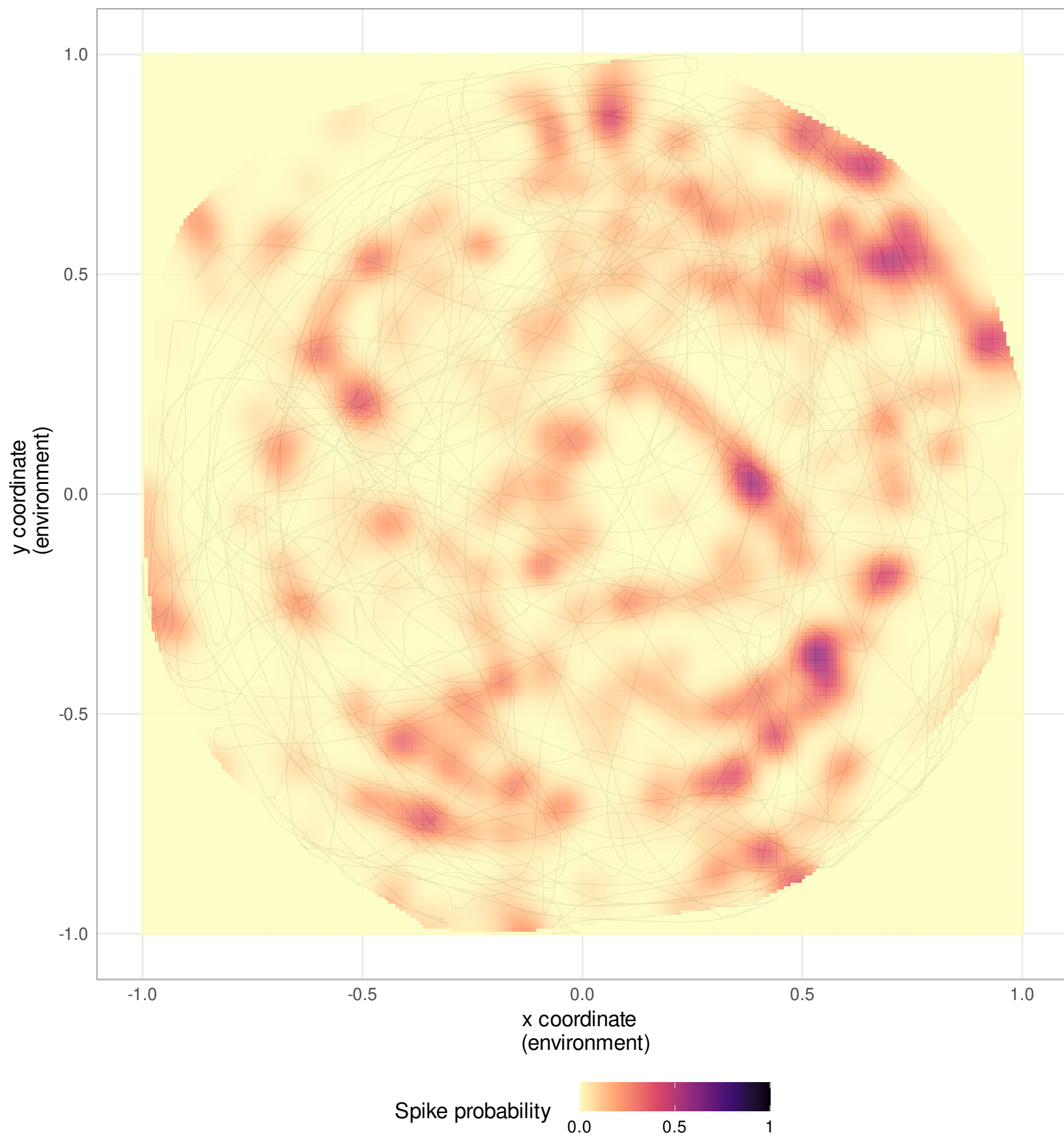
Neuron 66
