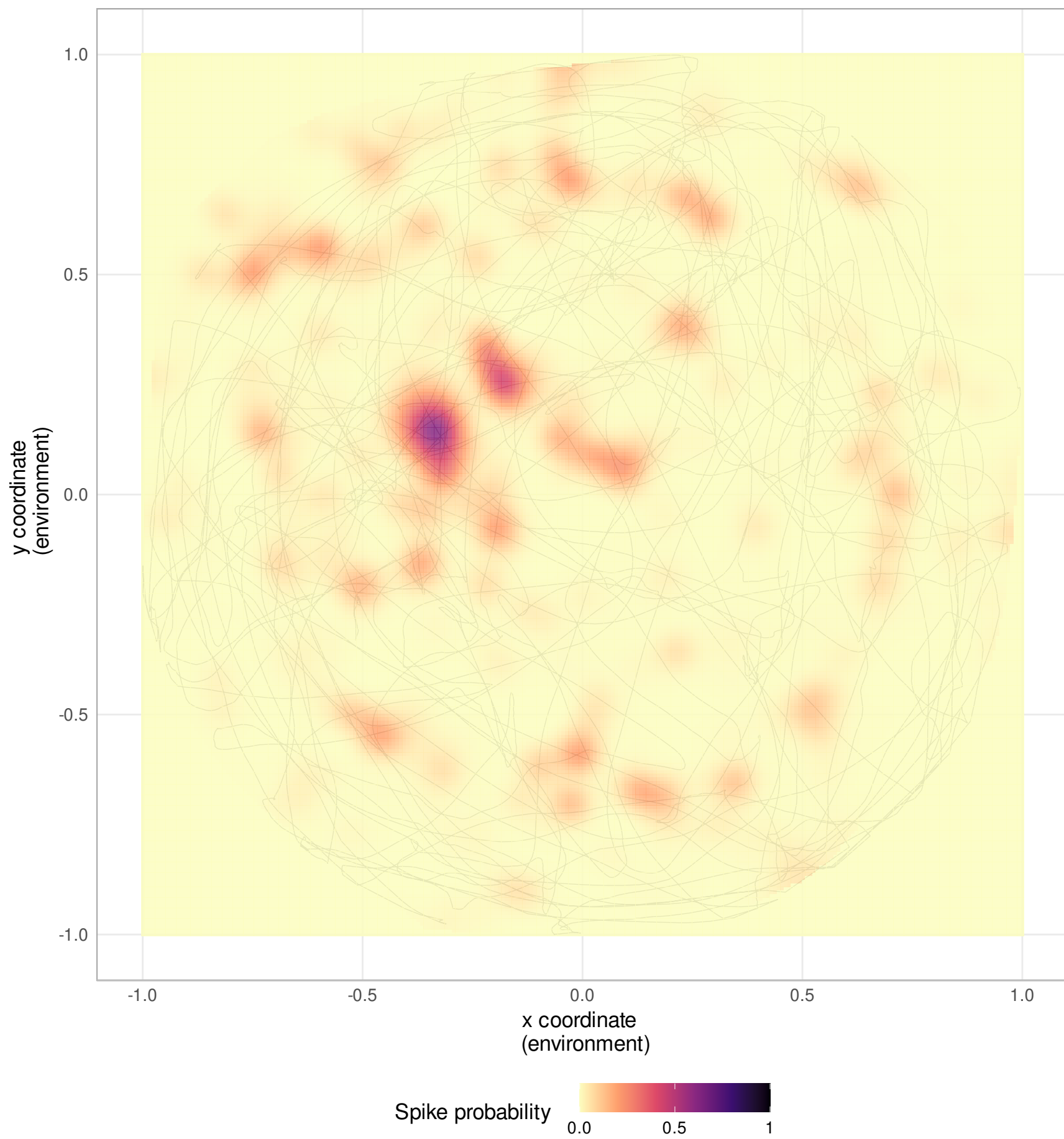
Neuron 67
