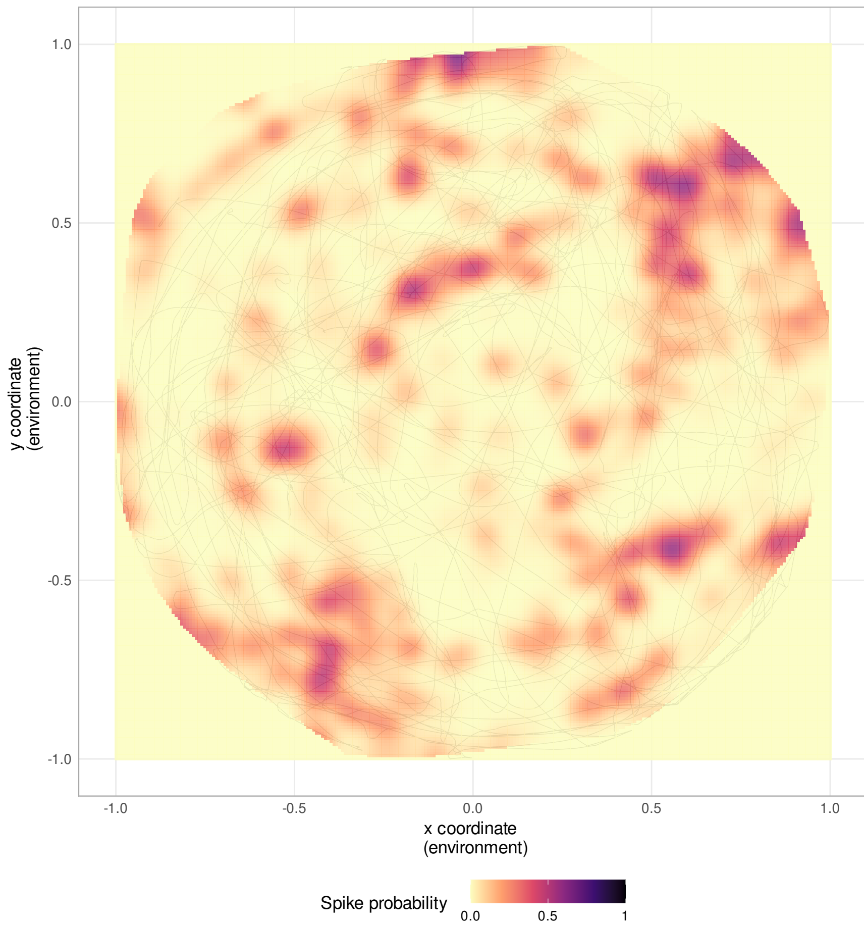
Neuron 69
