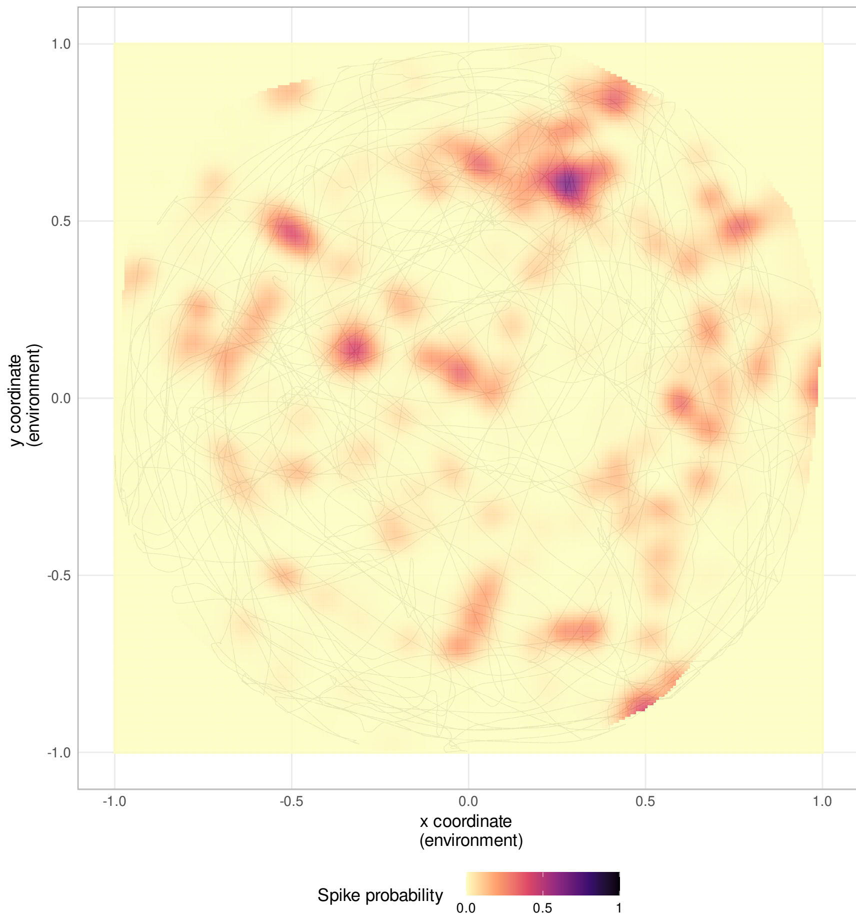
Neuron 71
