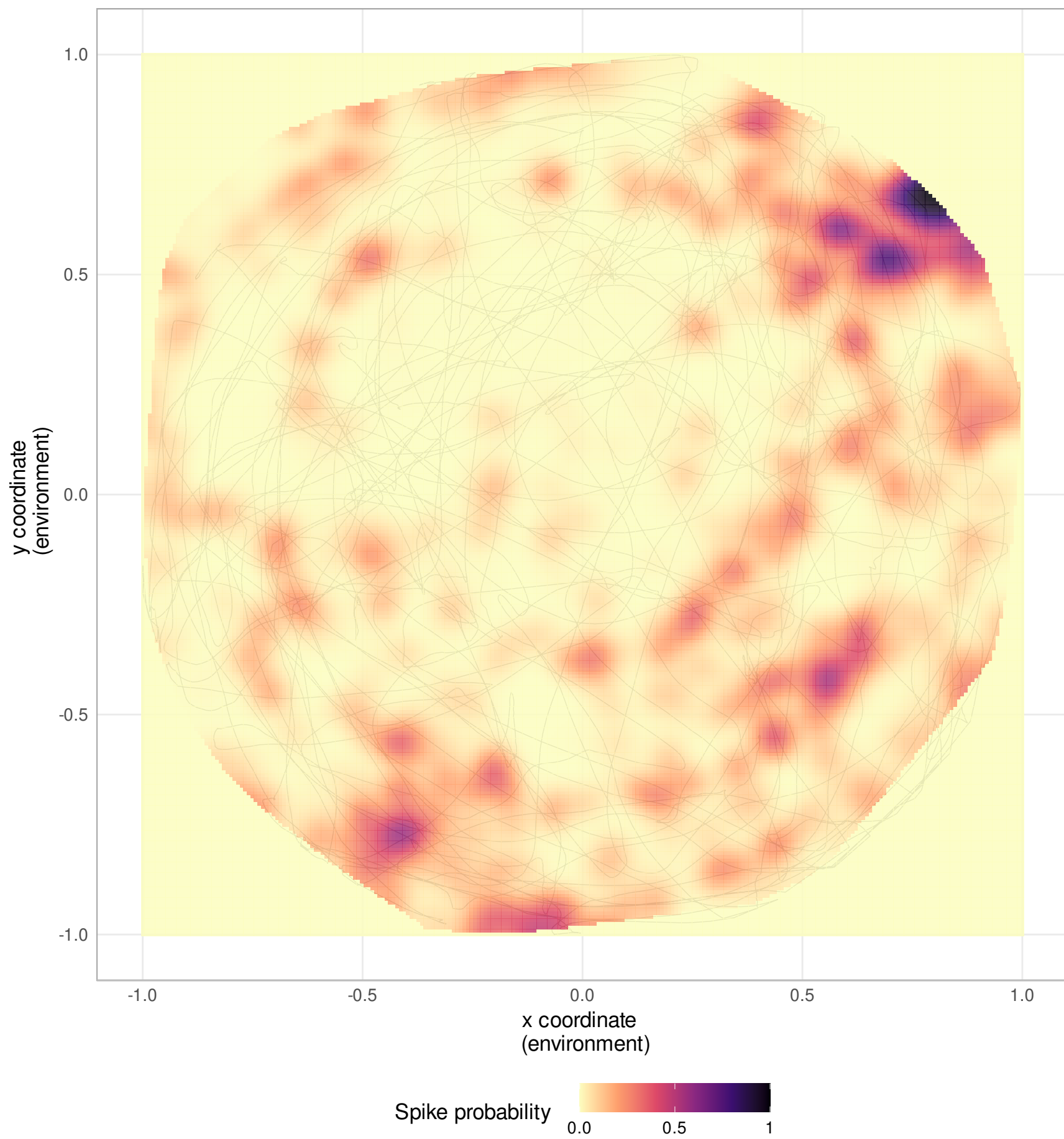
Neuron 73
