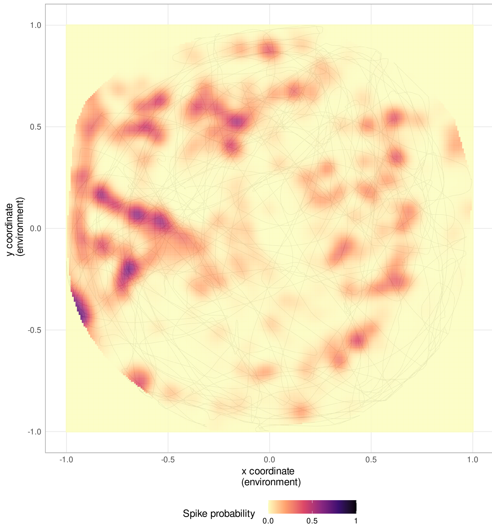
Neuron 75
