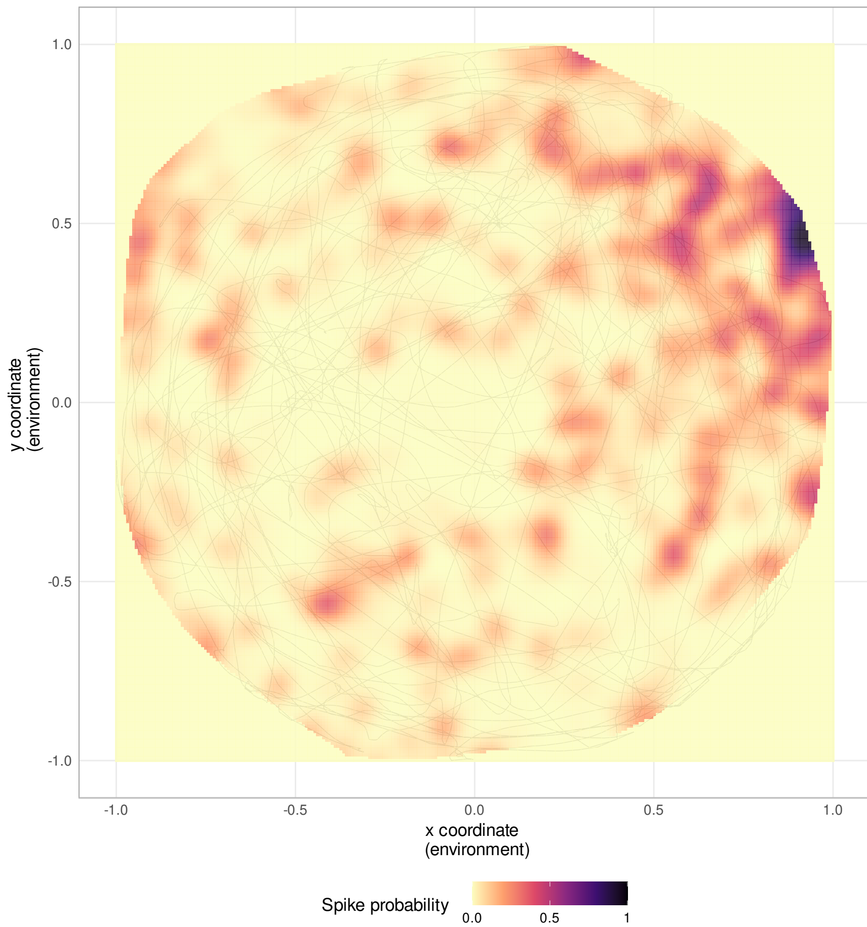
Neuron 78
