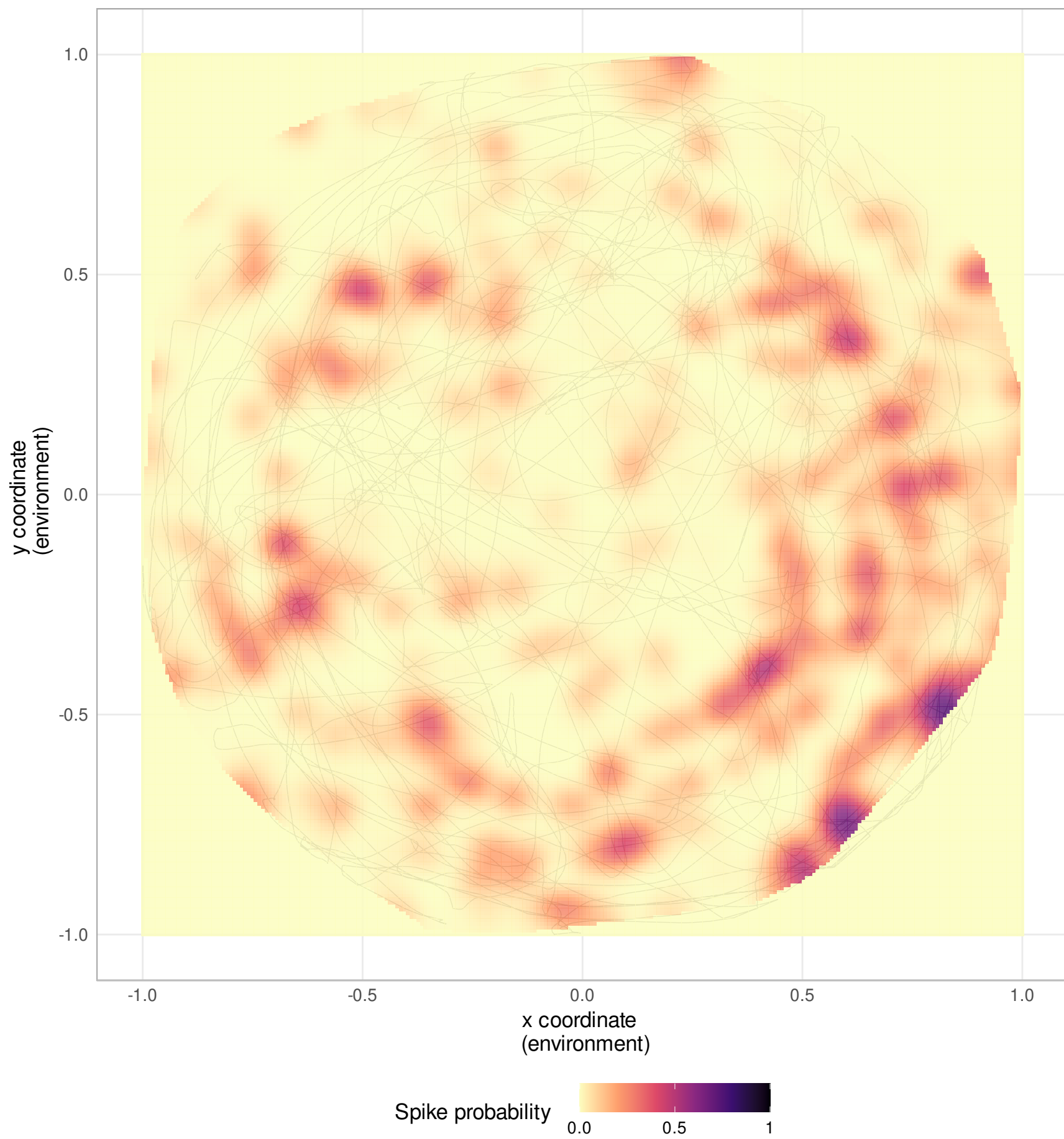
Neuron 79
