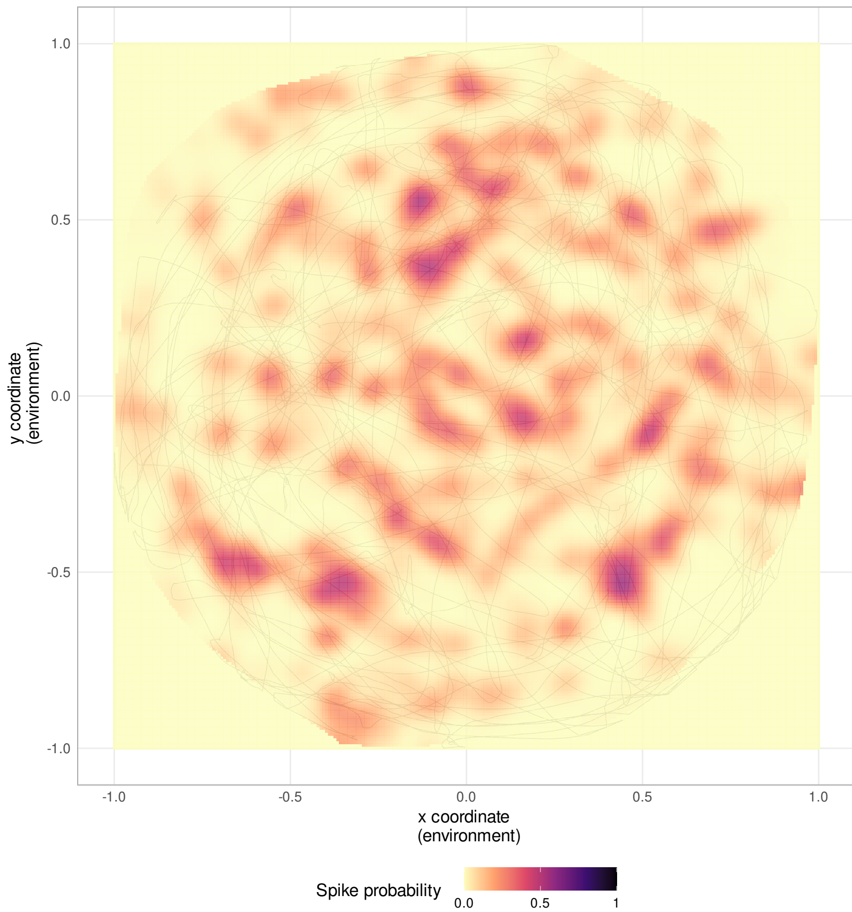
Neuron 83
