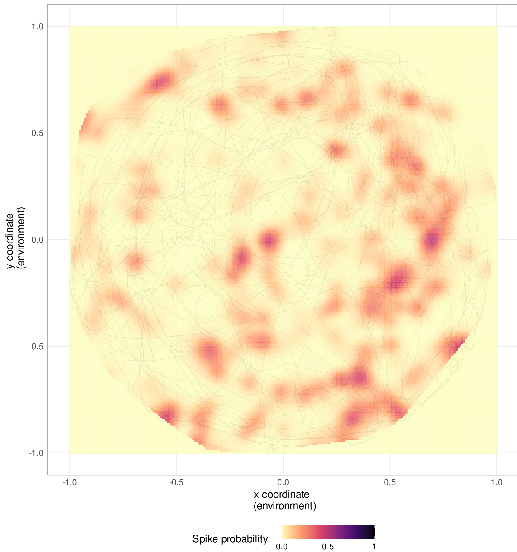
Neuron 86
