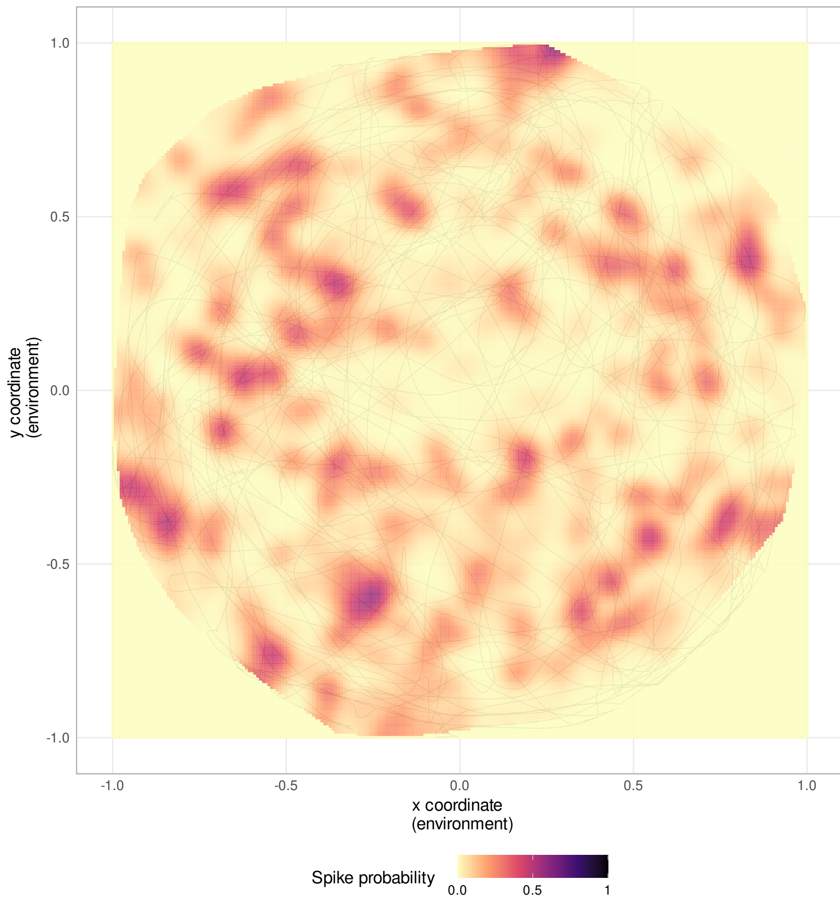
Neuron 91
