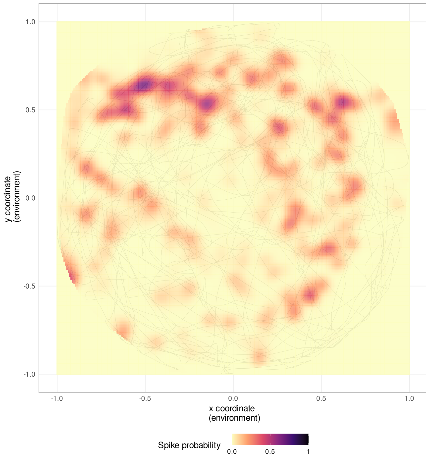
Neuron 94
