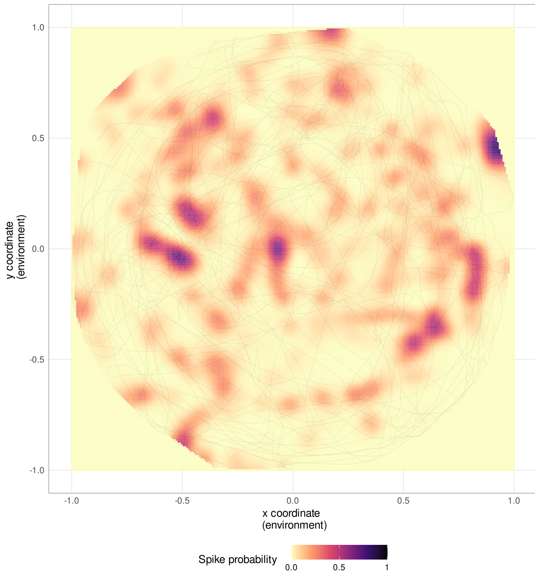
Neuron 98
