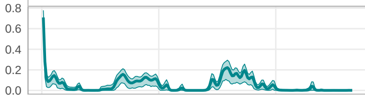
Cluster 2
