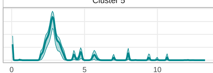
Cluster 5
