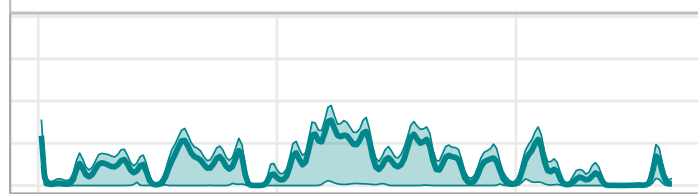
Cluster 3
