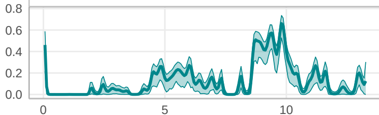
Cluster 6
