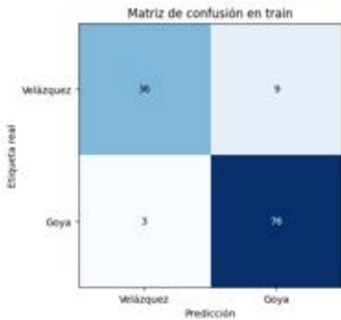
Figura 14: ViT train.
