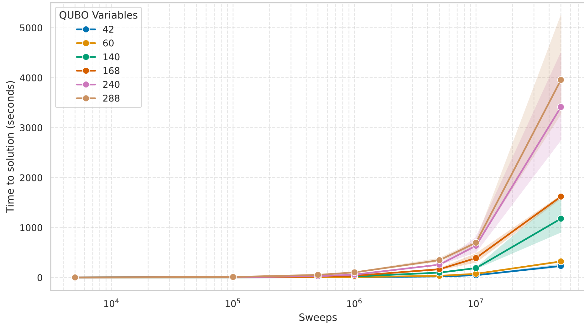
Time to solution vs. Sweeps - Classical Annealing (SA)
