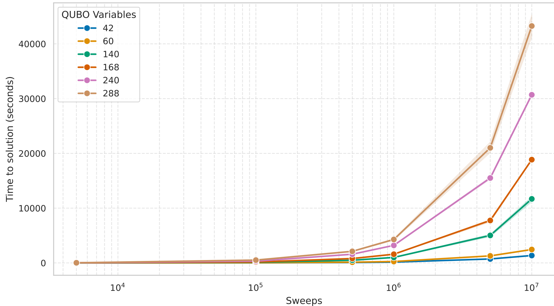
Time to solution vs. Sweeps - Quantum Annealing (QSA)
