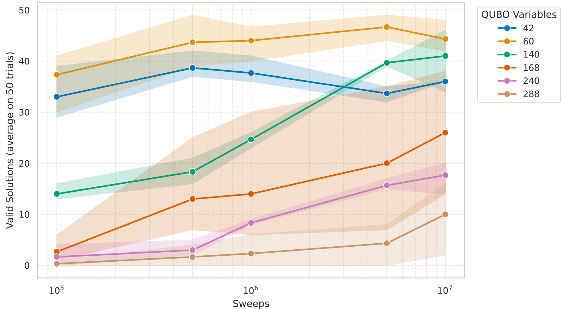
Valid Solutions vs. Sweeps - Quantum Annealing (QSA)
