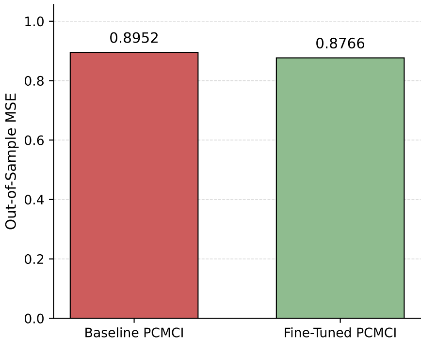
Prediction Error on Held-Out Data
