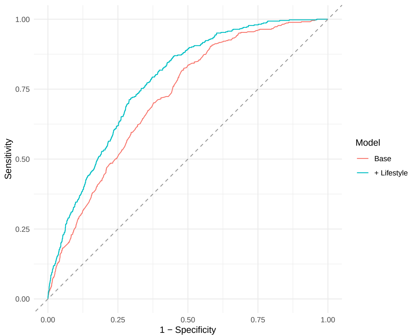
ROC: base vs. full model
