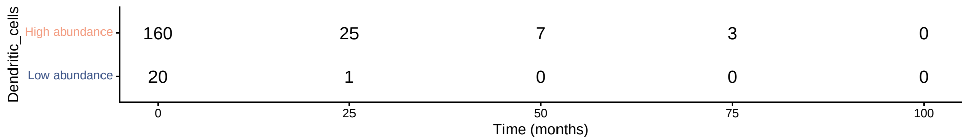
Number at risk
