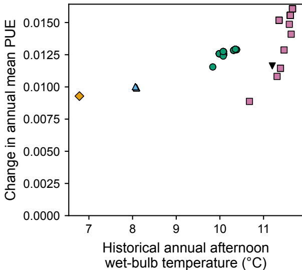
(b) PUE response, Case 1
