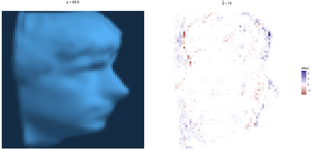
Figure 2: Left: Image corresponding to one observation in the Isomap faces data set. Right: The effect of each pixel \hat{\beta}_j^{1se} x_{i,j}^{new} in predicting the face orientation in left panel.
