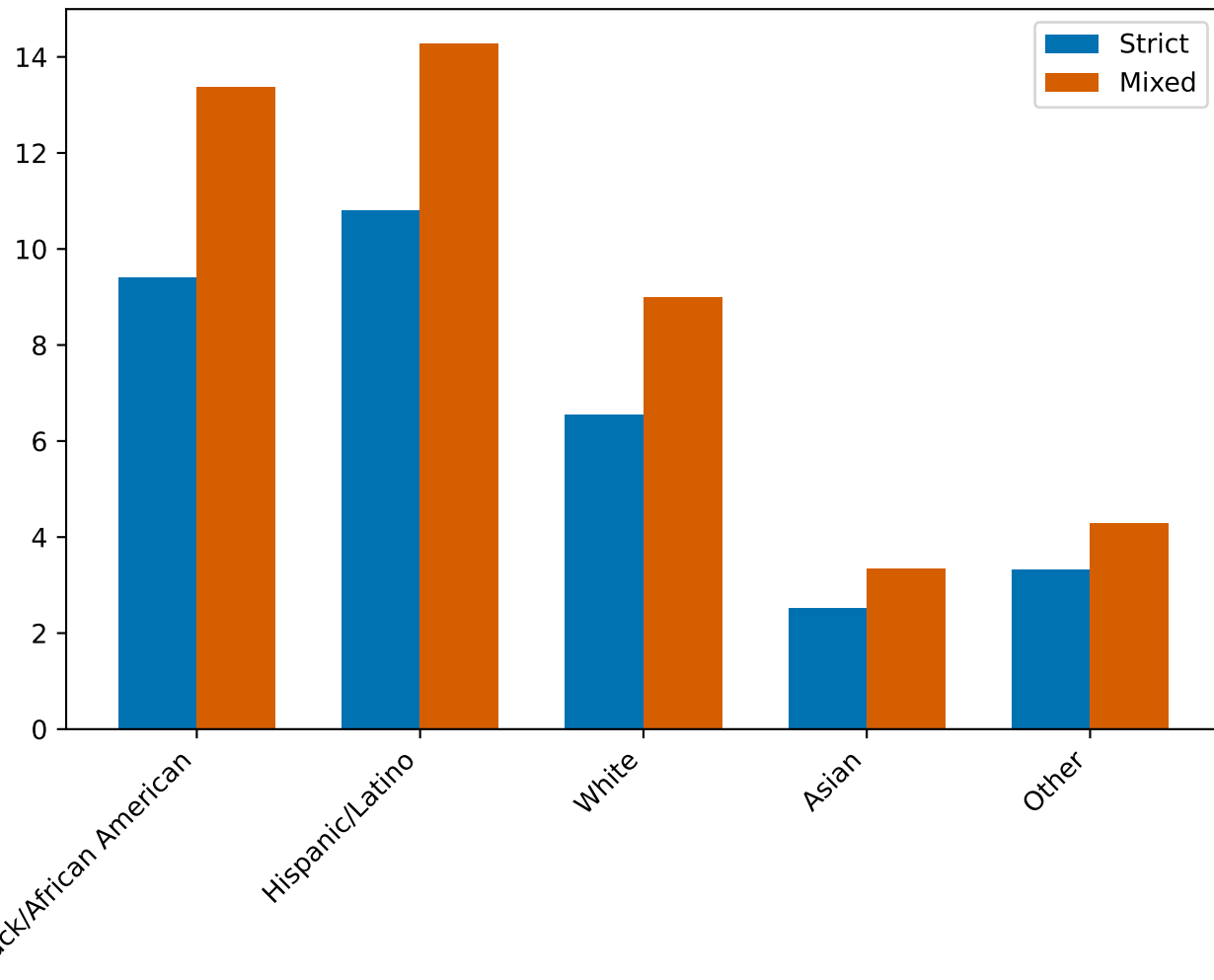
Search Rate (%)
