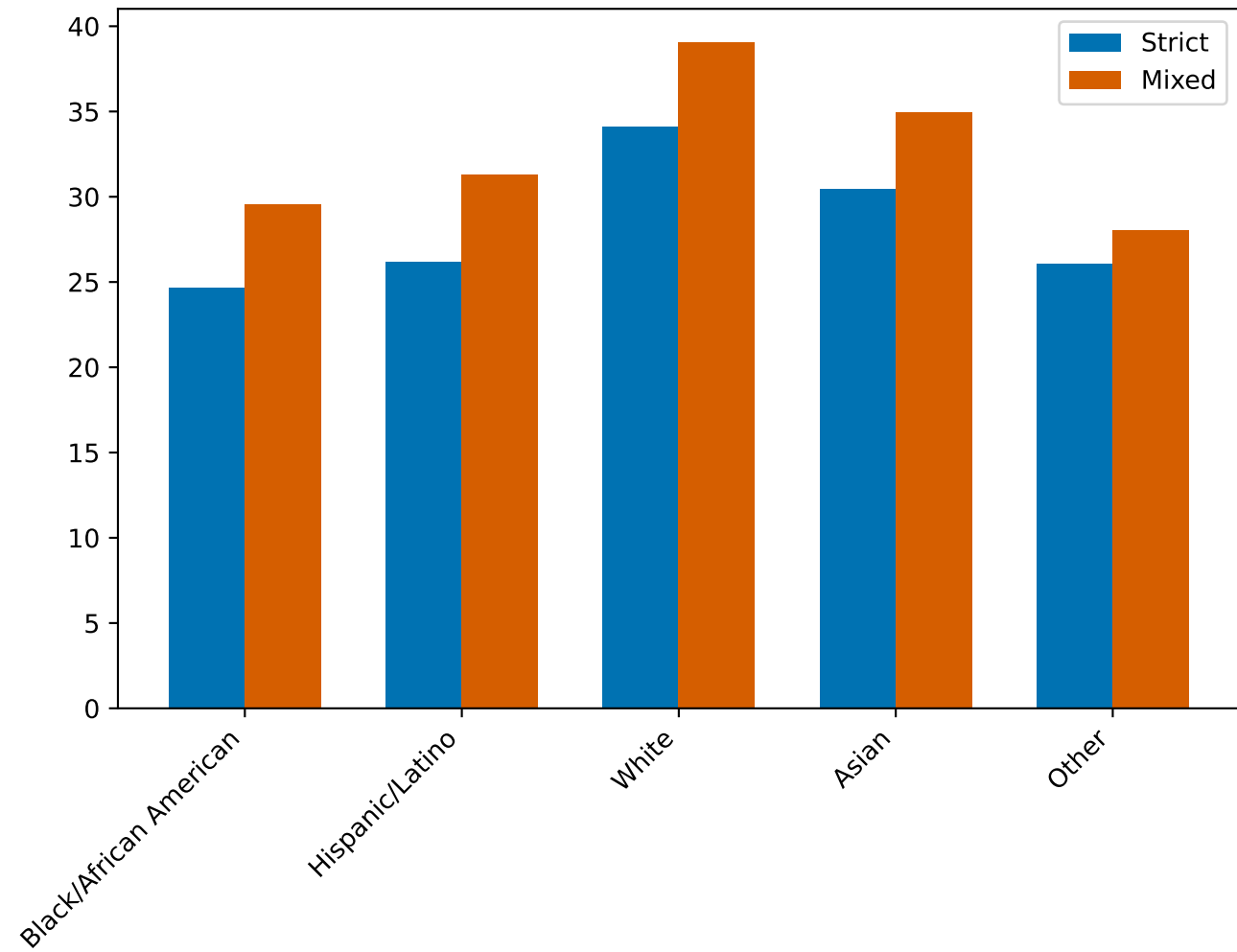
Hit Rate (%)
