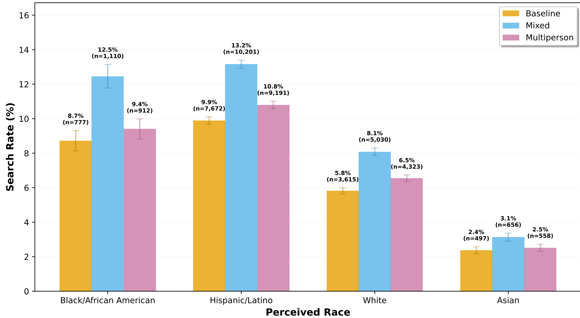
(A) Conditional Search Rate
