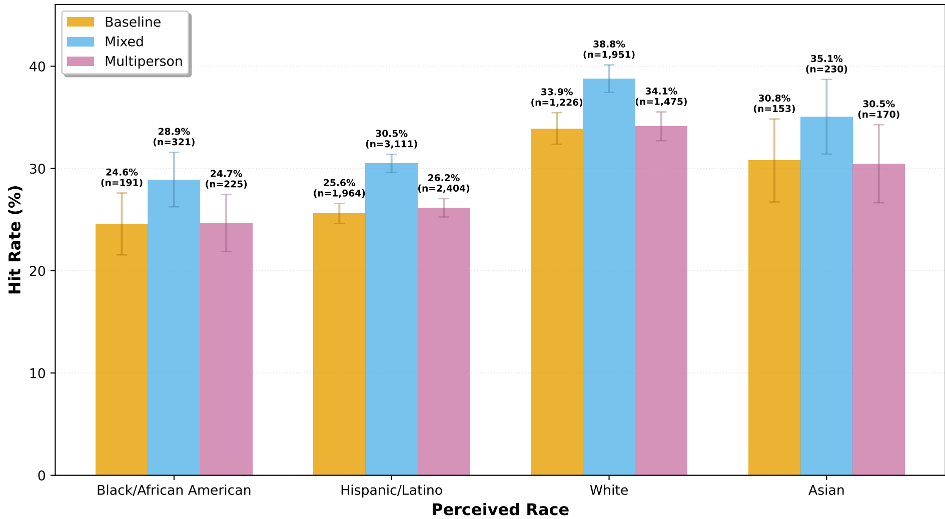
(B) Contraband Hit Rate
