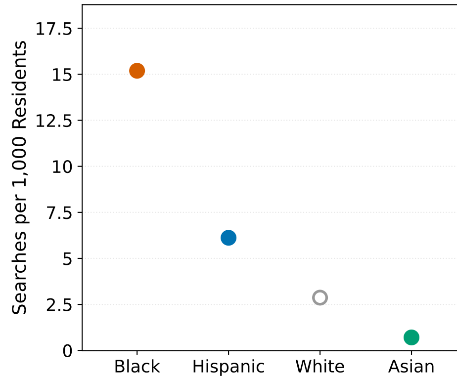
(B) Search Rate (per 1,000 residents)
