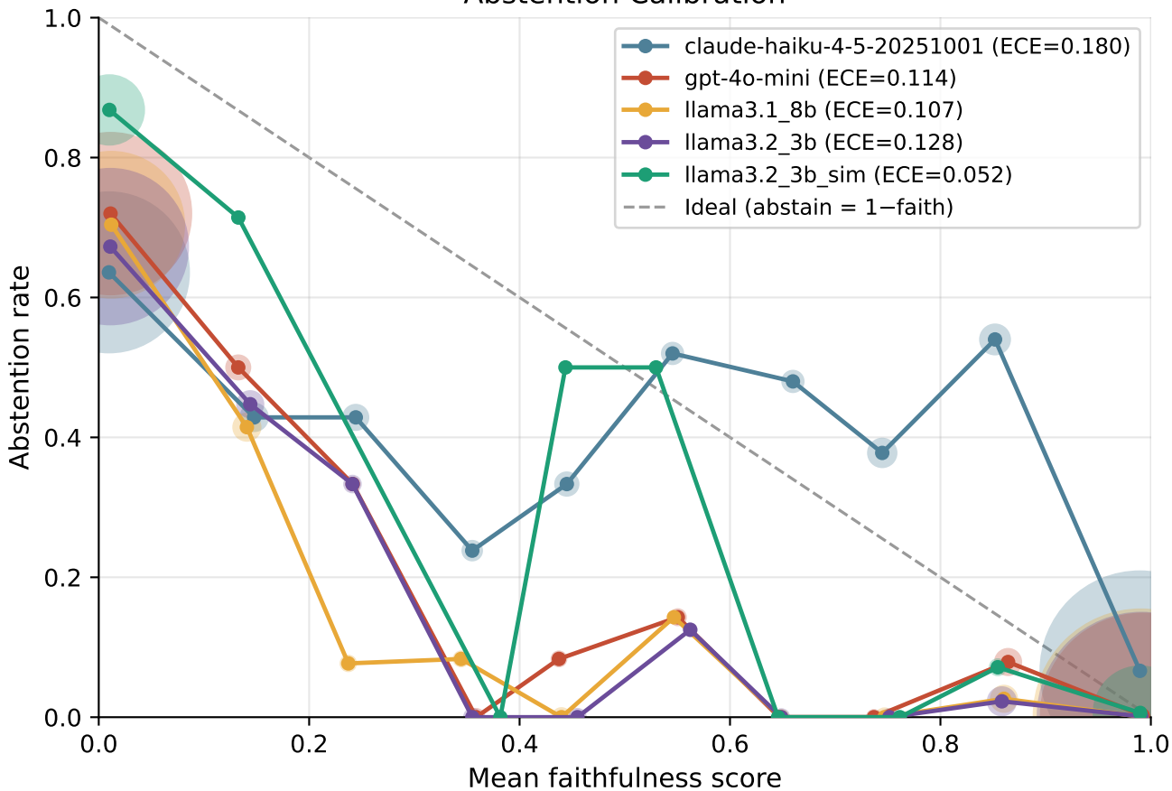
Abstention Calibration
