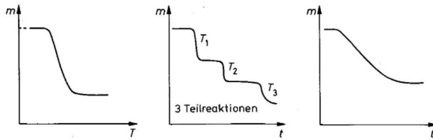
Figure 6: The diagramm on the left visualizes the mass plotted against the temperature. The other two show the mass plotted against time. [polyskript]
