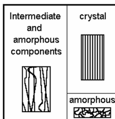
Figure 4: The figure shows possible structural elements of the polymer chains. [wunderlich_structure_2005]
