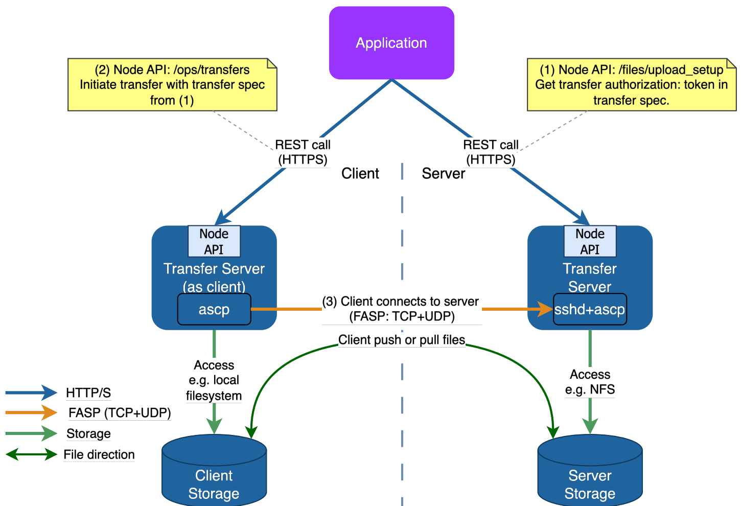
Figure 4.6: S6: server-to-server transfer with Node API and transfer token
