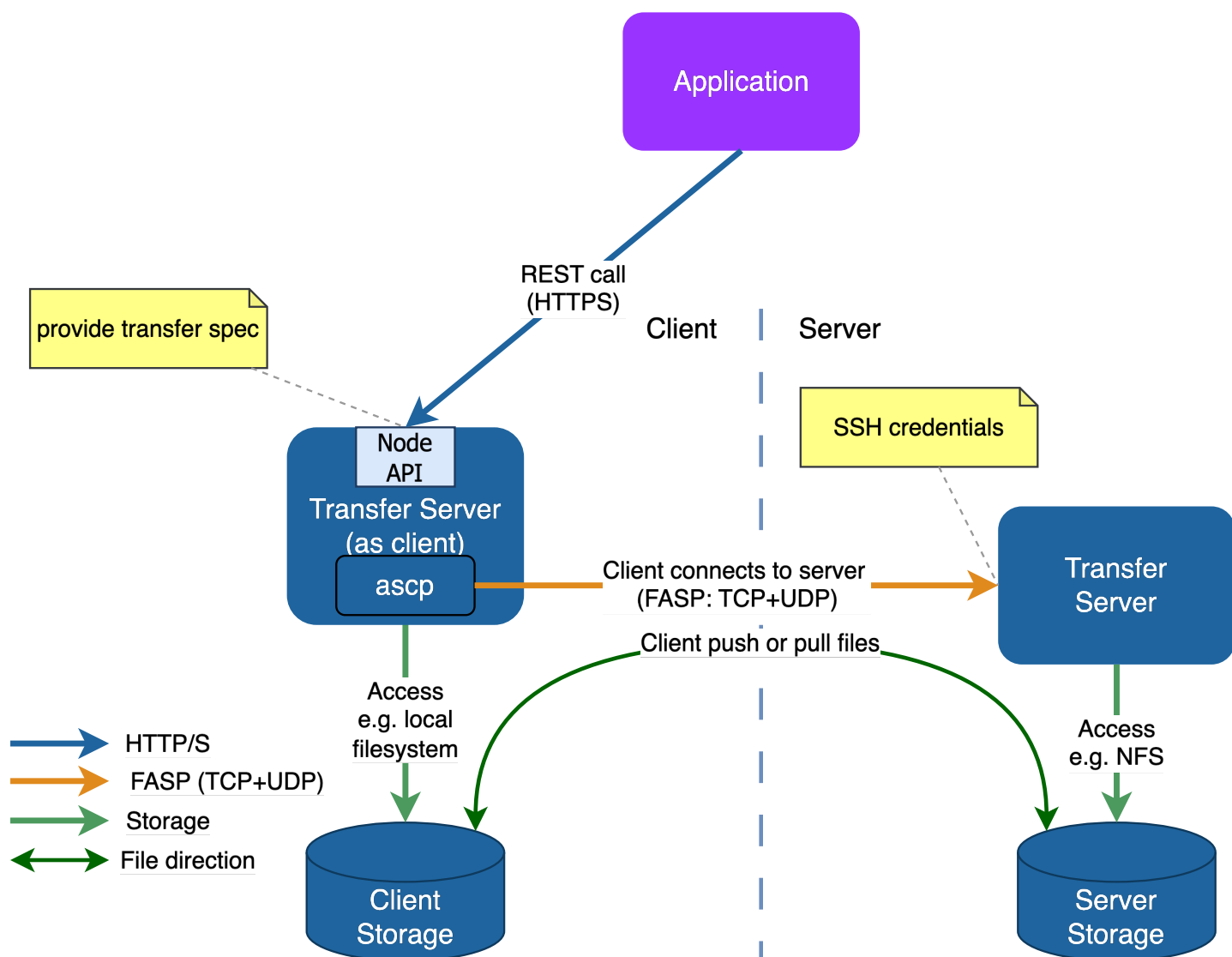
Figure 4.4: S4: server-to-server transfer with Node API and SSH credentials
