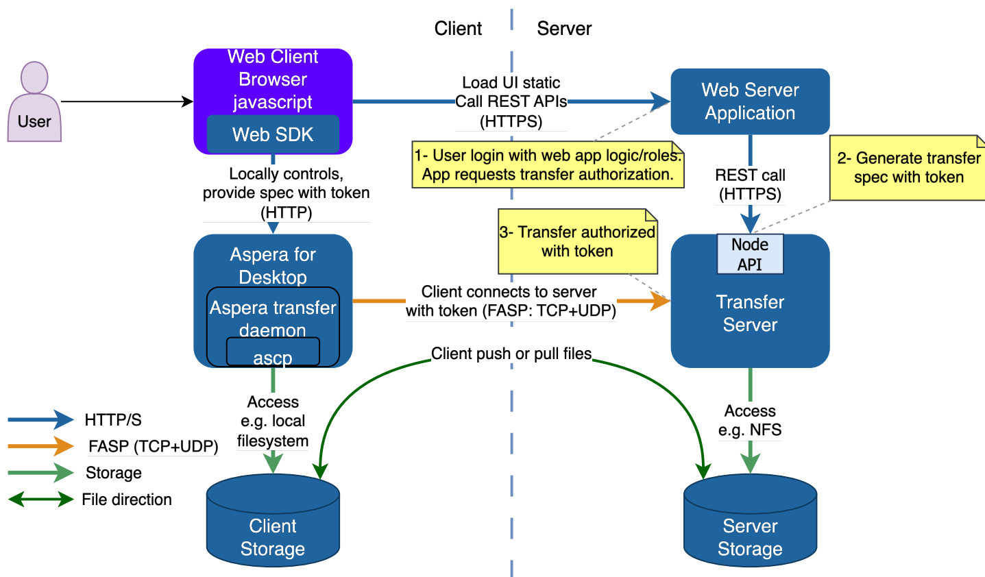
Figure 4.3: S3: web browser with Web SDK and token authorization
