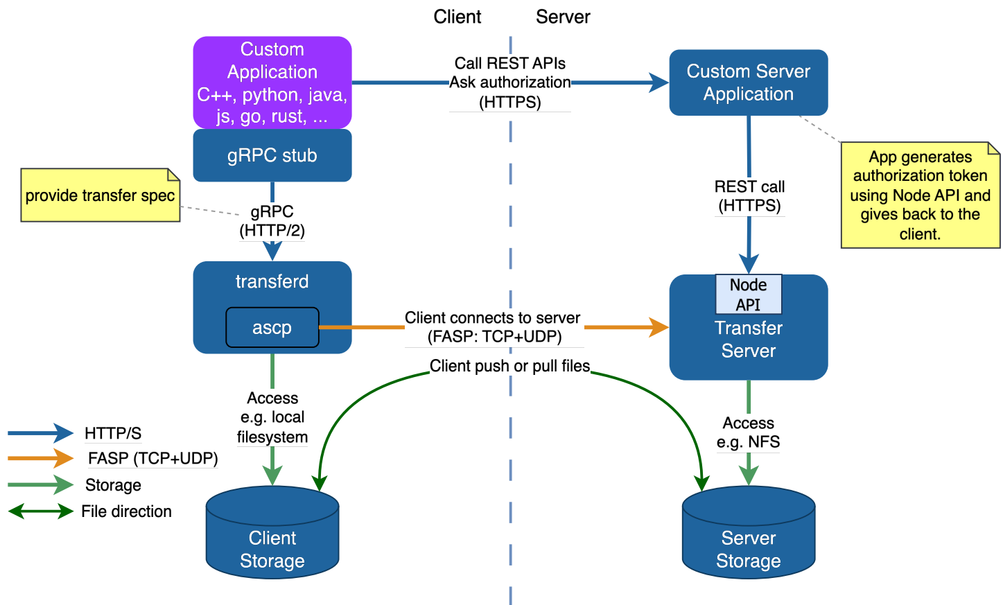
Figure 4.5: S5: custom client and server applications with token authorization
