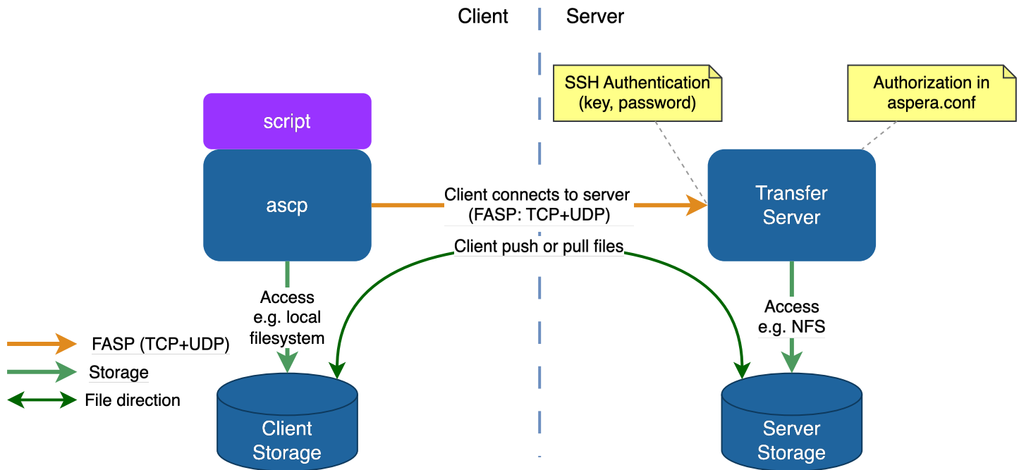
Figure 4.1: S1: script with ascp and SSH credentials
