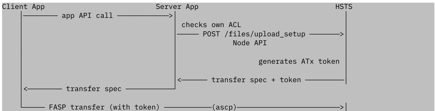
Figure 5.1: A2: Aspera transfer token authorization
