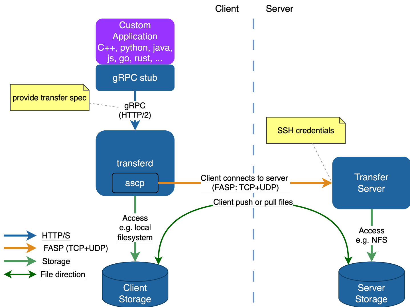
Figure 4.2: S2: custom application with Transfer Daemon and SSH credentials
