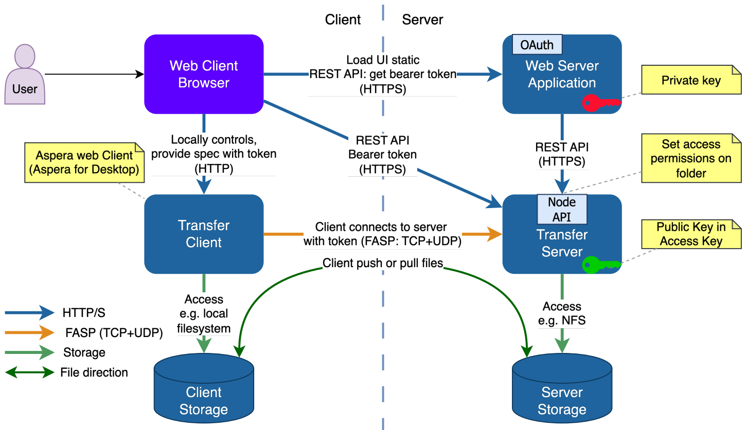
Figure 5.2: A3: Bearer token authorization
