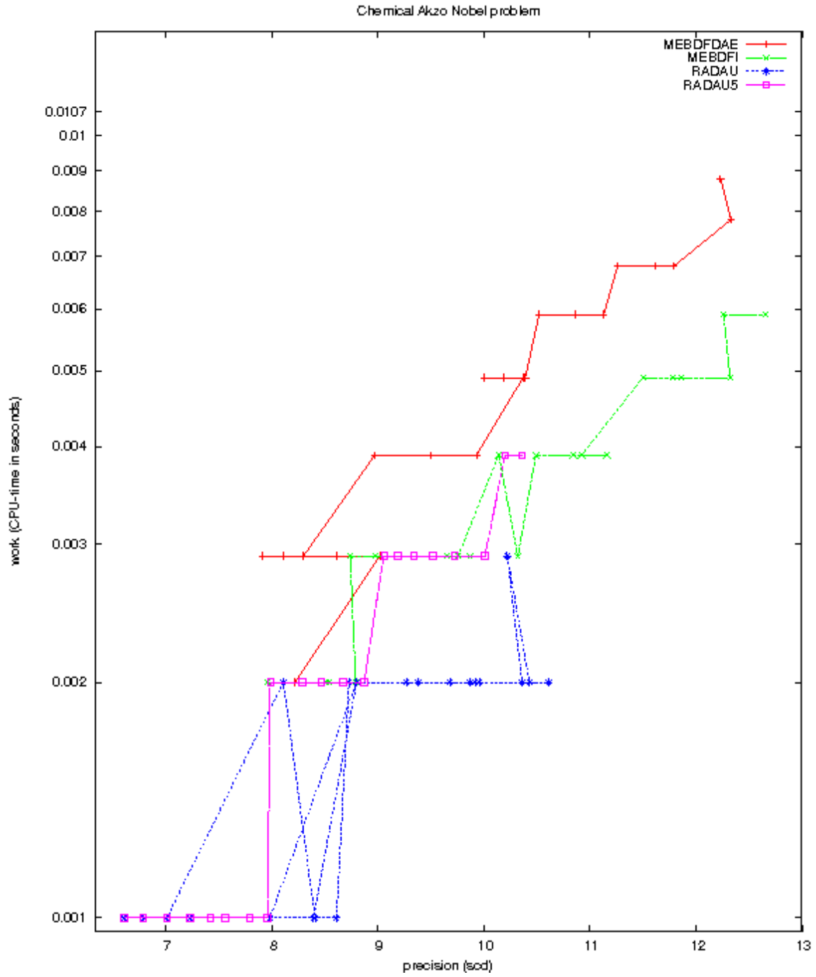
FIGURE II.12.4: Work-precision diagram (scd versus CPU-time).
