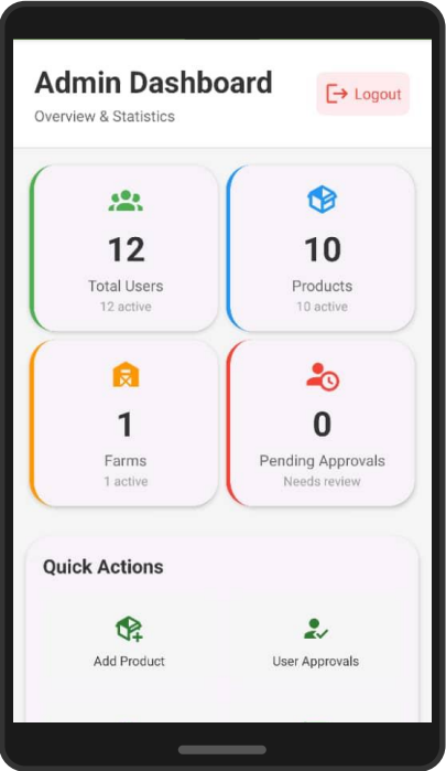
Admin Dashboard
