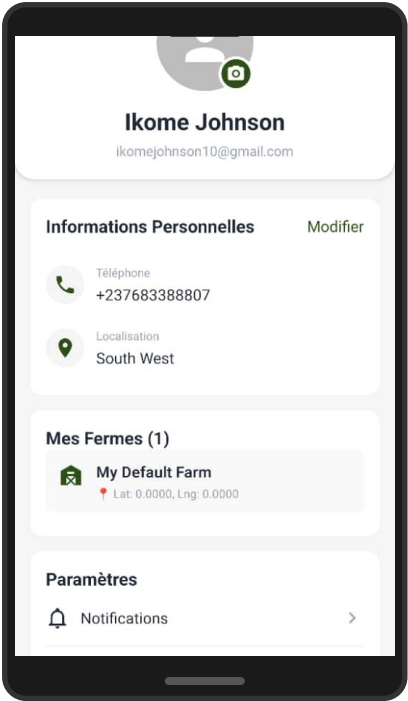
My Profile
