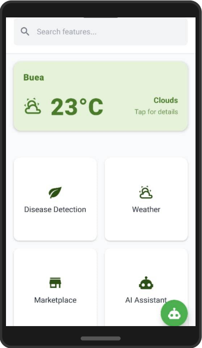
Home Screen
