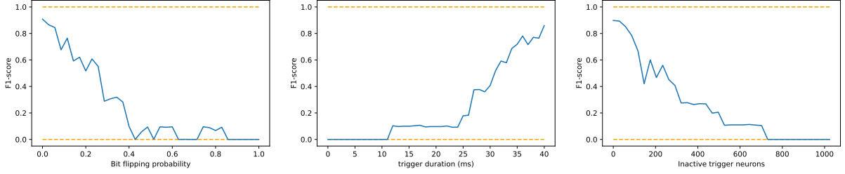
Figure 5: Robustness of working-memory retrieval to three types of trigger-window perturbation ( F_1 score averaged over M = 16 patterns). Left: Bit-flip noise applied to all spikes in the trigger window ( p_{\text{flip}} \in [0, 1] ); the network maintains high F_1 up to p_{\text{flip}} \approx 0.4 . Middle: Truncated trigger window (trigger duration from 0 to D - 1 = 40 steps); retrieval remains reliable for durations above roughly D/2 . Right: Partial neuron coverage (number of silenced neurons from 0 to N = 1024 ); perfect recall is maintained until the majority of the trigger population is inactive. Orange dashed lines indicate F_1 \in \{0, 1\} .
