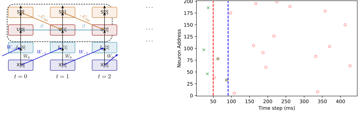
Figure 2: Network architecture and a sample target pattern. Left : Unrolled view of the recurrent HD-SNN over time (one column representing one time step), illustrating delayed connections between neurons: Blue arrows indicate synaptic connections that integrate past activity across heterogeneous delays; for clarity only one delay is shown. Right : One representative target spike pattern ( N = 1024 neurons, T = 1000 time steps, of which we show 256 neurons and 400 time steps); each red circle marks one target spike. The goal of the network is to memorise M = 16 such patterns. Each trial is flanked by N_{\text{pretime}} = 50 time steps of spontaneous background activity (random spikes at rate p_A ) before and after the stimulus. The trigger window (green crosses between the dashed lines) consists of the first D = 41 time steps of the target pattern clamped to the network input; the recurrent network then autonomously predicts the remaining spikes.
