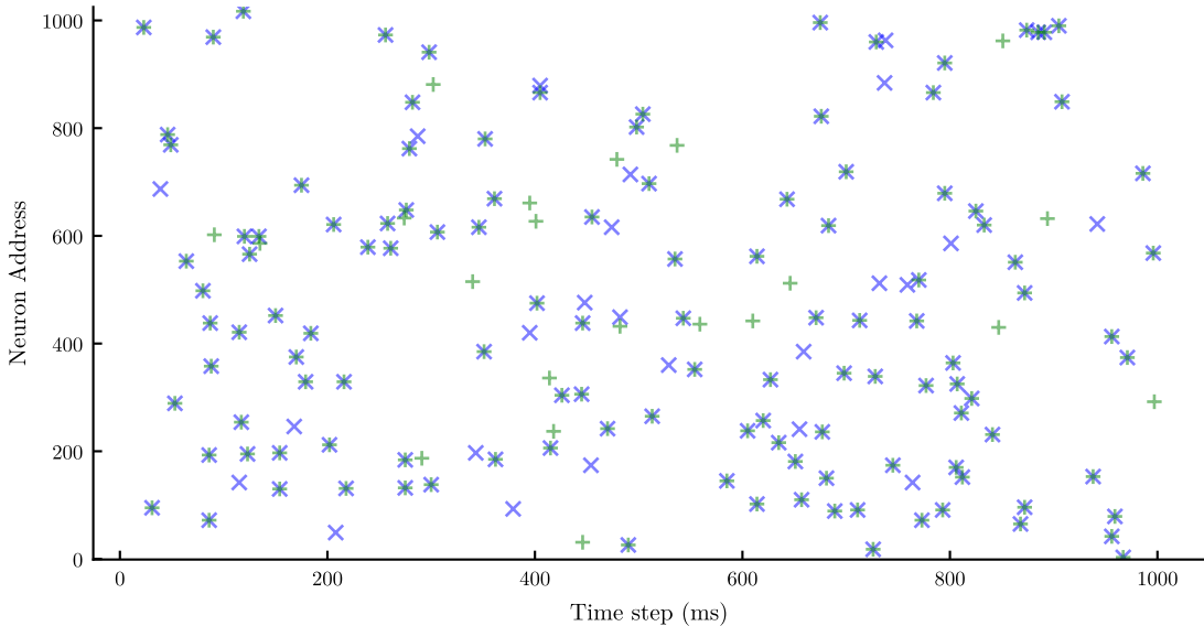
Two instances of a Stochastic Spiking Pattern ssp.opt.p_flip=0.10
