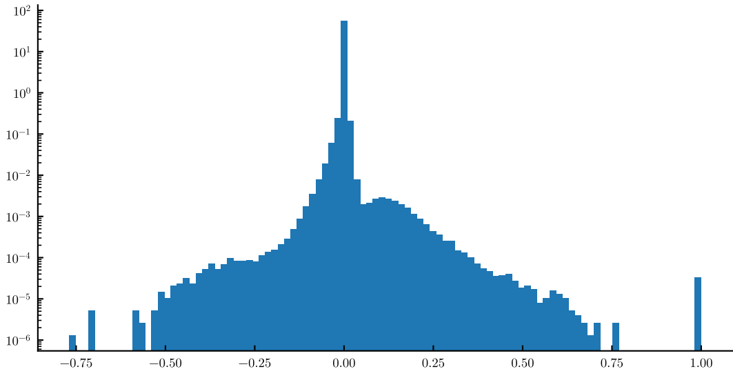
Histogram of the HD-SNN weights after learning
