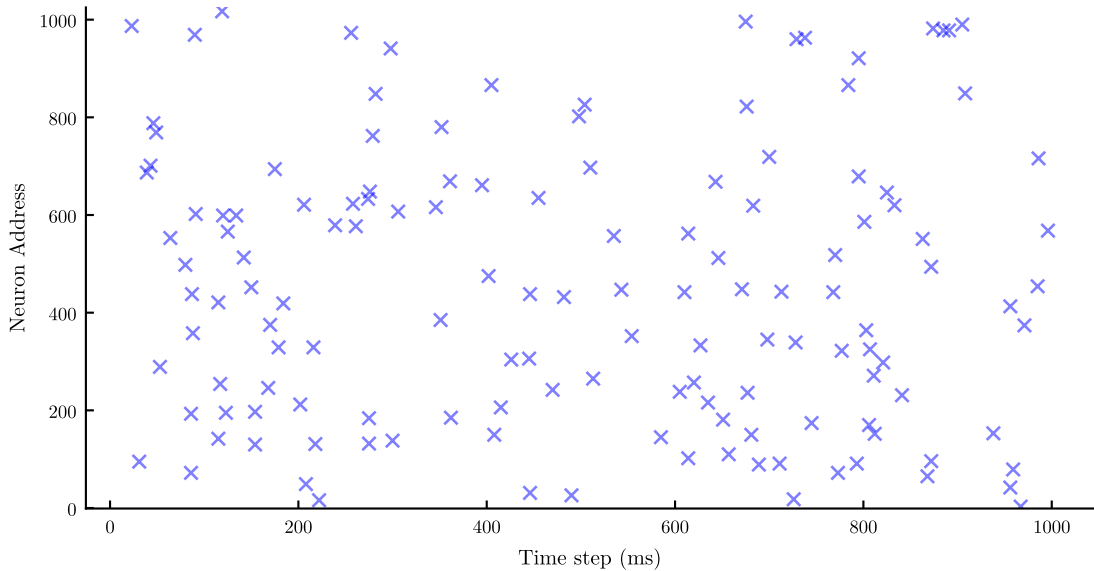
Frozen Spiking Pattern 0 (sum=140.0)
