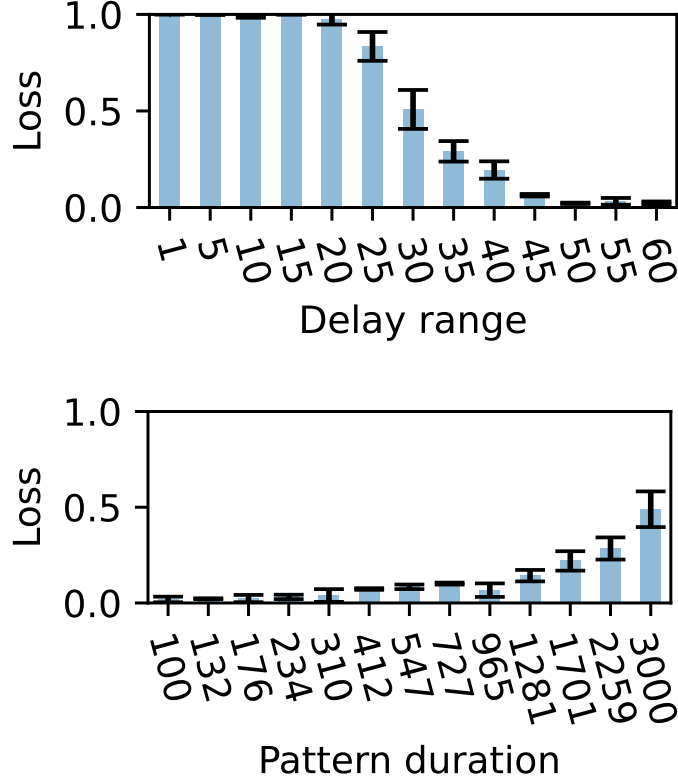
Figure 6: Effect of some key parameters on working-memory performance (loss \mathcal{L} = 1 - F_1 , mean \pm s.e. over N_{cv} = 10 cross-validation folds). Left : Increasing the maximum delay D consistently reduces the loss, confirming that deeper delay windows provide a larger, more orthogonal context and that longer maximum delays directly increase the capacity of the recurrent HD-SNN. Right : Loss grows slowly and monotonically with pattern duration T , consistent with the compounding-error and gradient-vanishing arguments: longer sequences require the network to maintain coherent predictions further from the trigger window.
