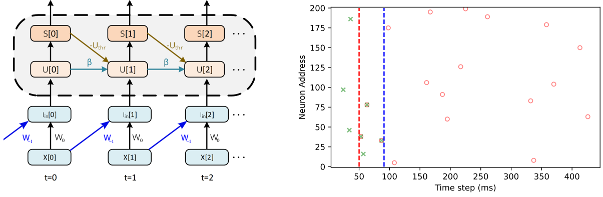
Figure 2: Network architecture and a sample target pattern. Left : Unrolled view of the recurrent HD-SNN over time (one column representing one time step), illustrating delayed connections between neurons: Blue arrows indicate synaptic connections that integrate past activity across heterogeneous delays; for clarity only one delay is shown. Right : One representative target spike pattern ( N = 1024 neurons, T = 1000 time steps, of which we show 256 neurons and 400 time steps); each red circle marks one target spike. The goal of the network is to memorise M = 16 such patterns. Each trial is flanked by N_{\text{pretime}} = 50 time steps of spontaneous background activity (random spikes at rate p_A ) before and after the stimulus. The trigger window (green crosses between the dashed lines) consists of the first D = 41 time steps of the target pattern clamped to the network input; the recurrent network then autonomously predicts the remaining spikes.
