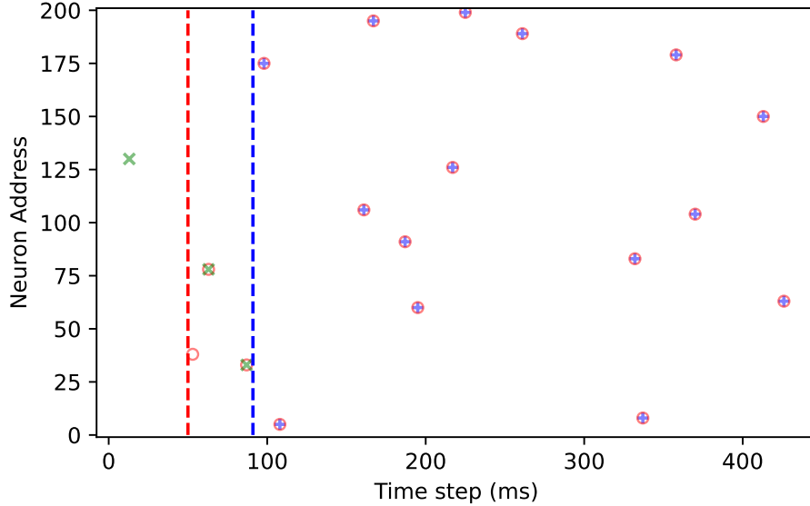
Fig. 3. Pattern retrieval from the recurrent HD-SNN. After clamping the network with input spikes (green crosses) with 50 steps of spontaneous activity (left of the red dashed line) and a trigger window consisting of the initial sequence of one of the M = 16 target patterns ( 0 \leq t < D = 41 , delimited by the dashed red and blue line), we simulate the network after training output the duration the full sequence duration ( T = 1000 steps). We observe that the raster plot shows network activity (blue crosses, N = 1024 neurons) which perfectly matches the target pattern which was cued during the trigger window. Note that the target spikes after the trigger window (red circles right of the blue dashed line) are hidden from the network.
