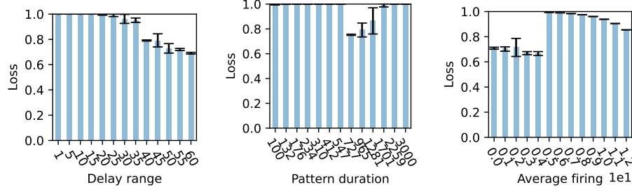
Fig. 5. Effect of three key parameters on working-memory performance (loss \mathcal{L} = 1 - F_1 , mean \pm s.e. over N_{cv} = 10 cross-validation folds). Left: Increasing the maximum delay D consistently reduces the loss, confirming that deeper delay windows provide a larger, more orthogonal context and that longer maximum delays directly increase the capacity of the recurrent HD-SNN. Middle: Loss grows slowly and monotonically with pattern duration T , consistent with the compounding-error and gradient-vanishing arguments: longer sequences require the network to maintain coherent predictions further from the trigger window. Right: Performance is optimal at low background firing rates ( p_A \lesssim 10^{-3} ) and degrades sharply at higher rates.
