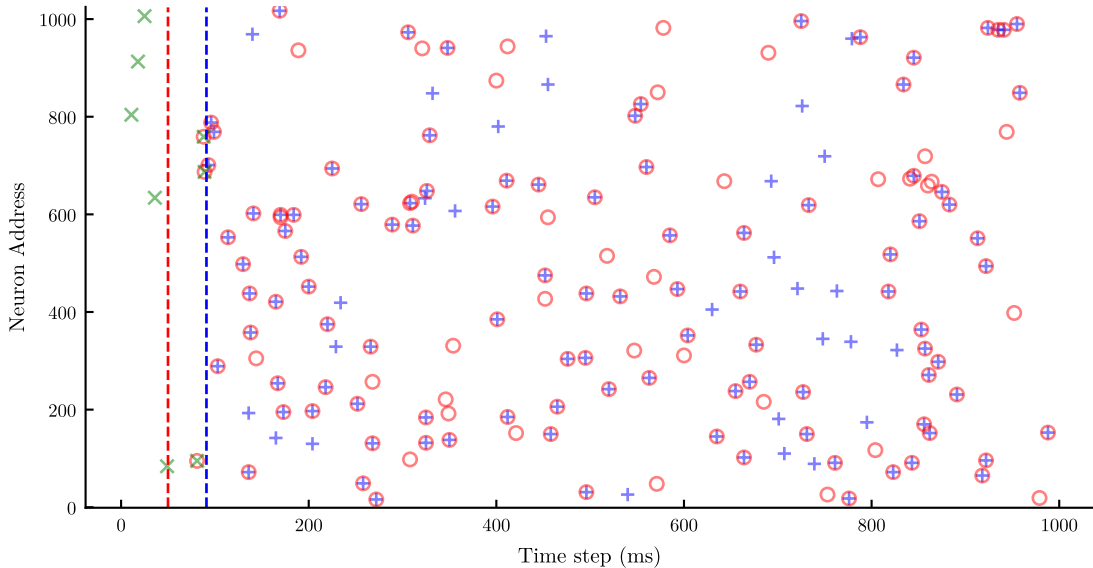
Inference with a noisy trigger p_{\text{flip}}=18\%
