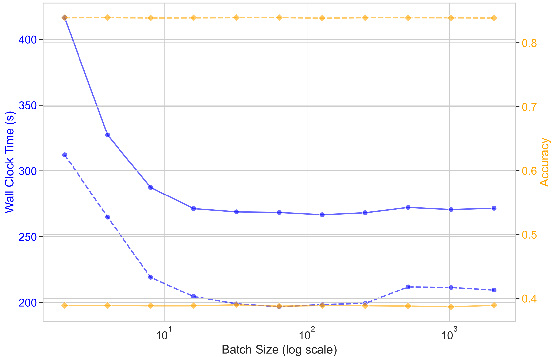
Model Performance vs. Batch Size
