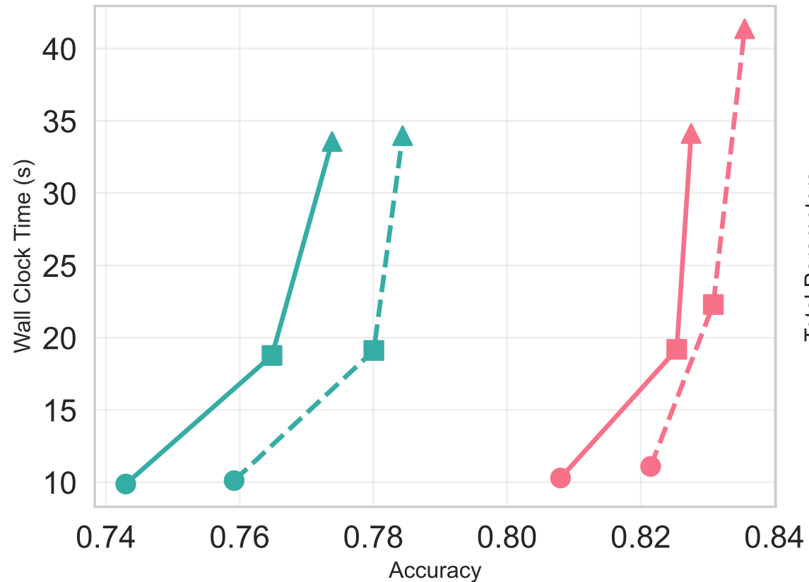
Inference Time vs Accuracy
