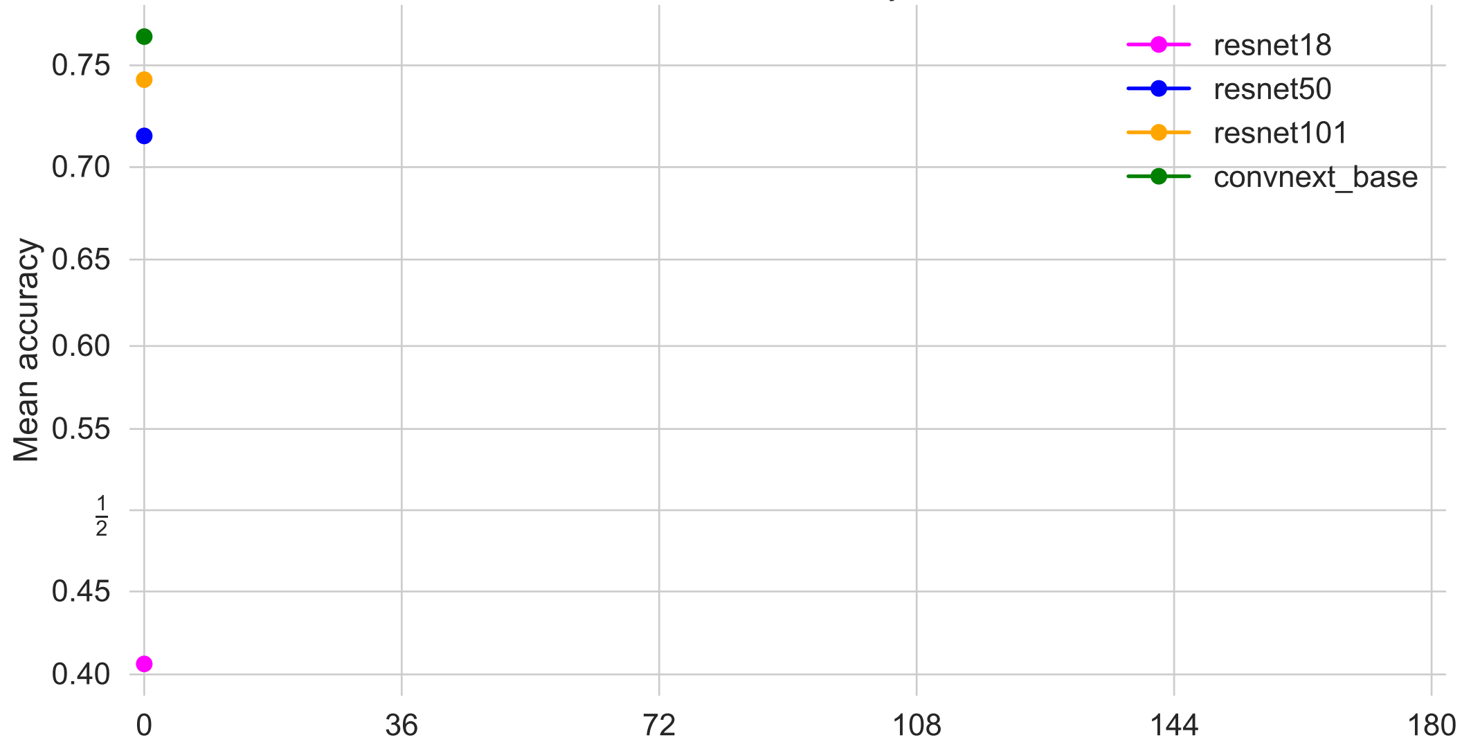
Model accuracy
