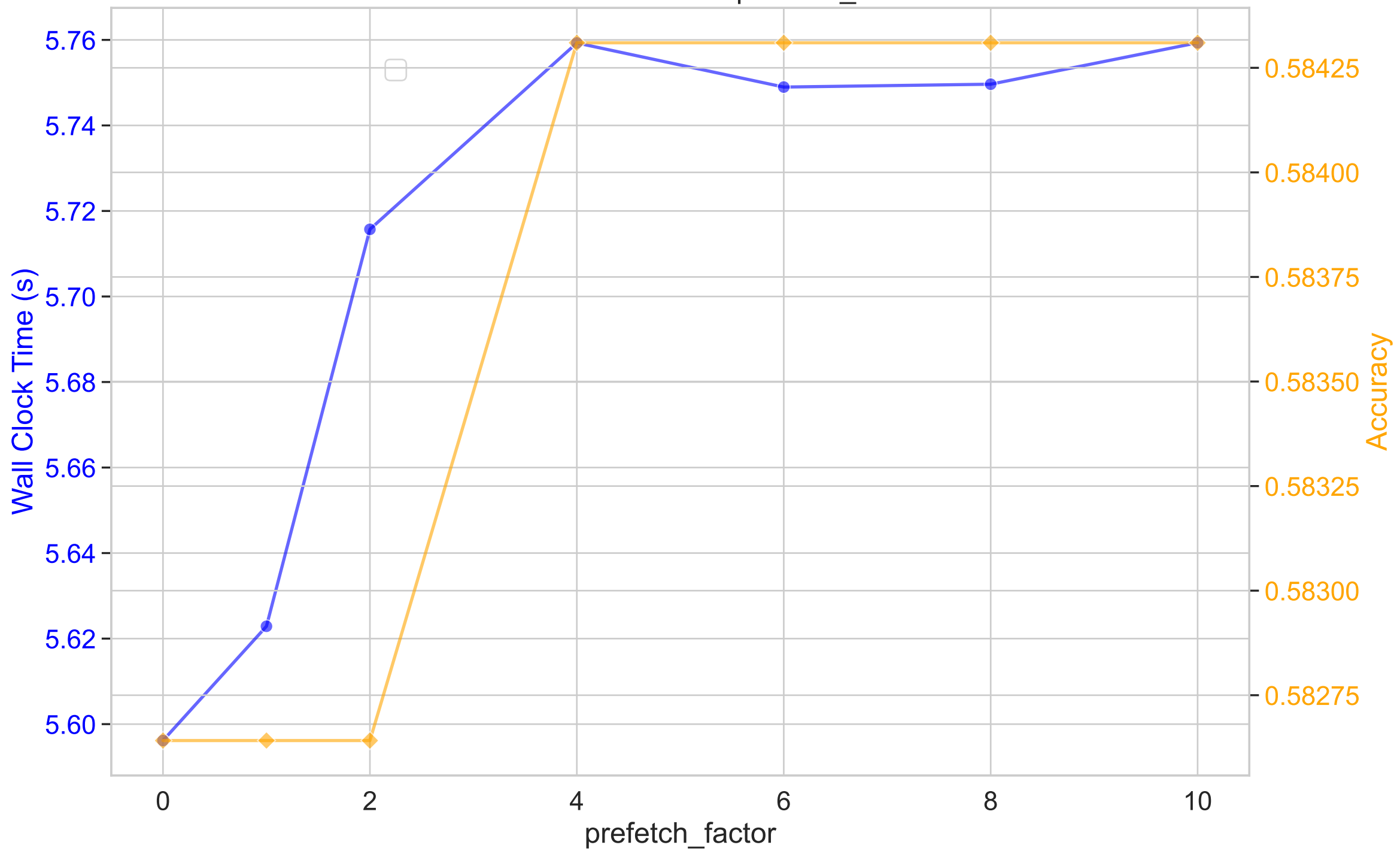
Model Performance vs. prefetch_factor
