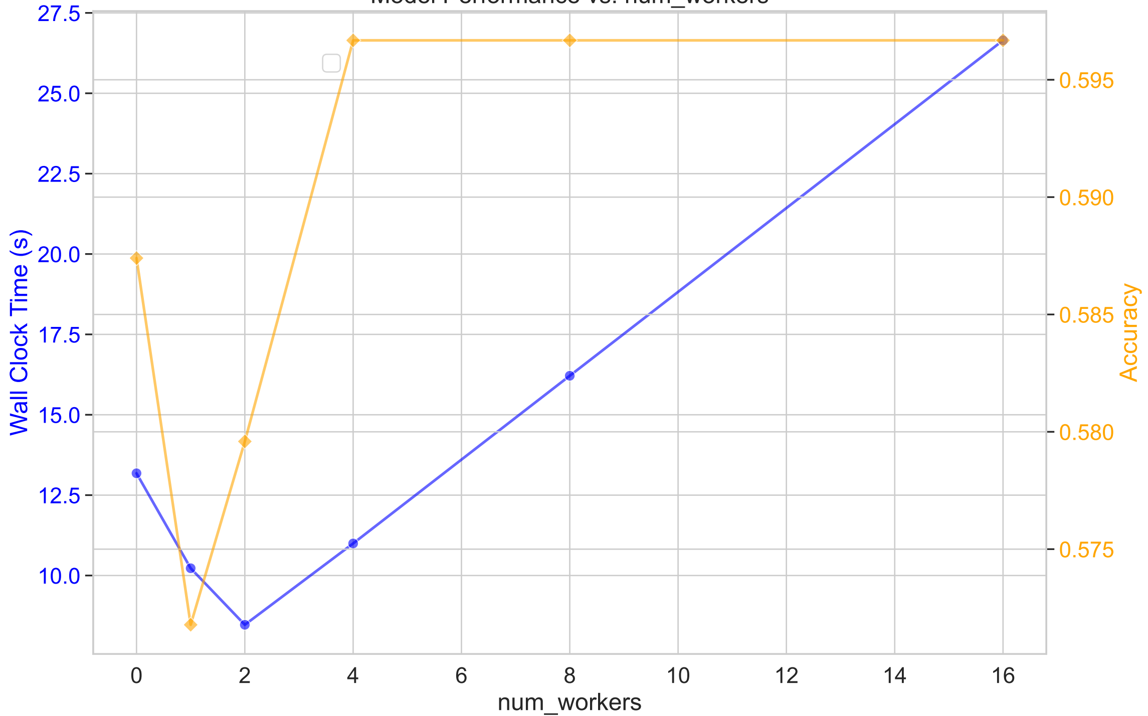
Model Performance vs. num_workers
