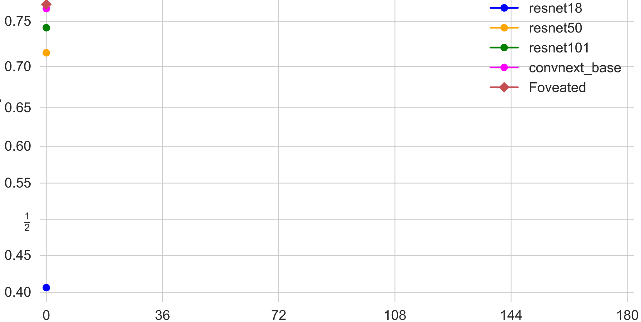
Model accuracy
