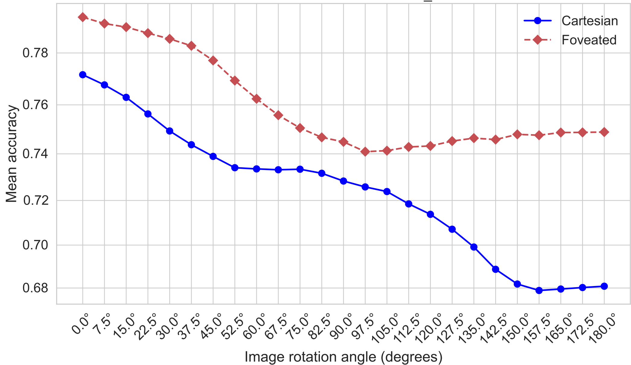
Model robustness to rotations: convnext_base on bbox
