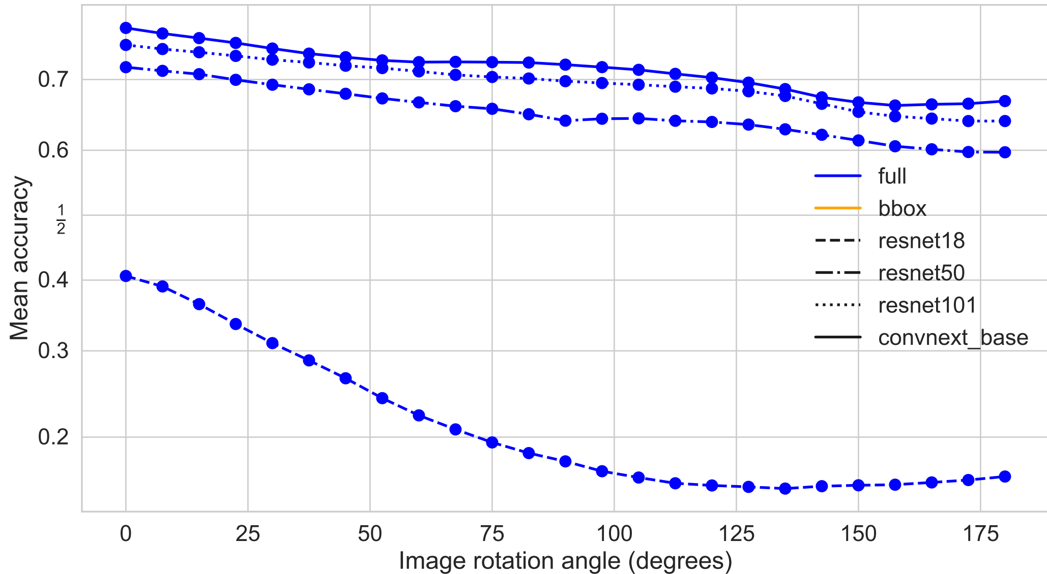
Model robustness to rotations
