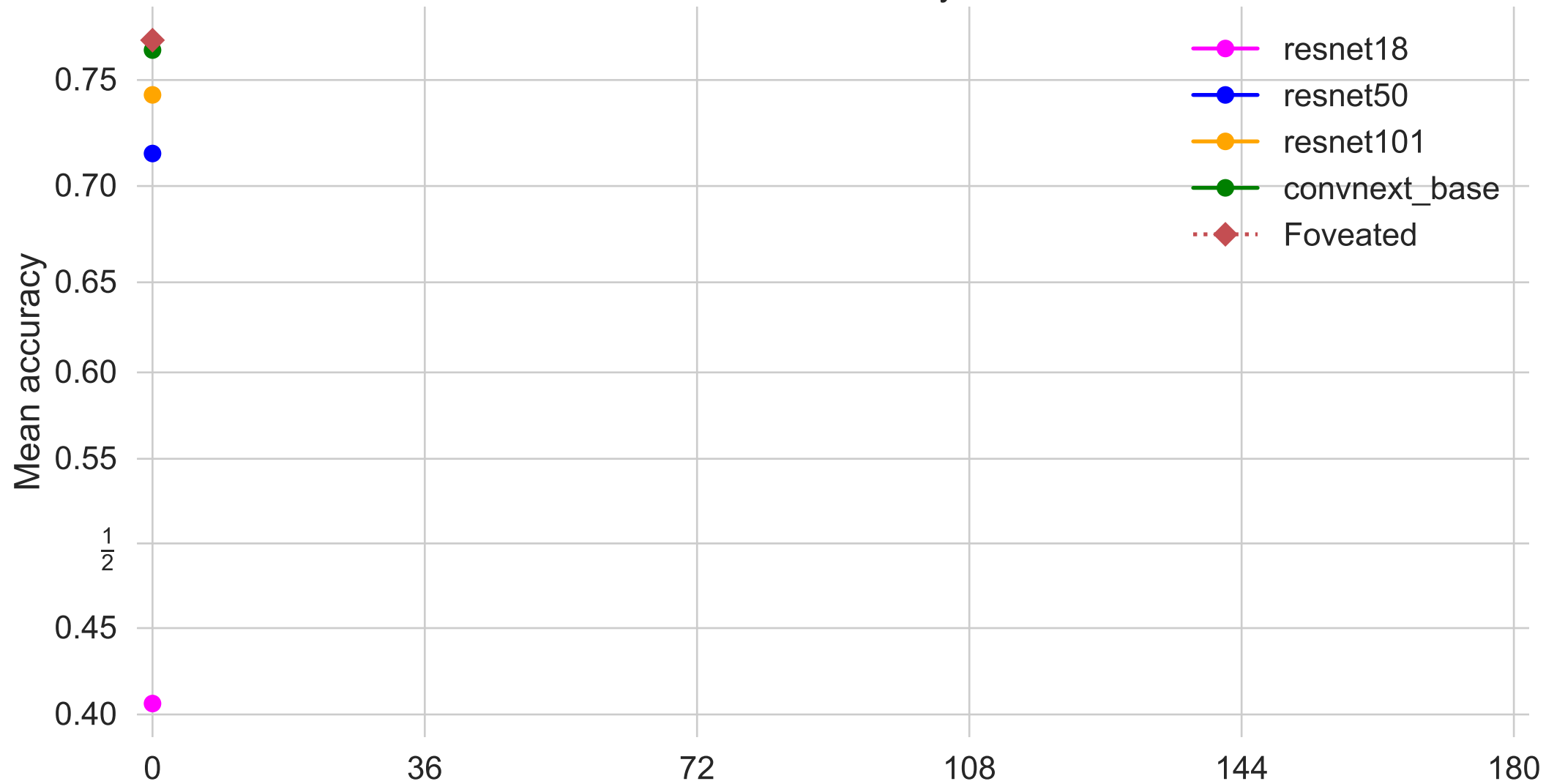
Model accuracy
