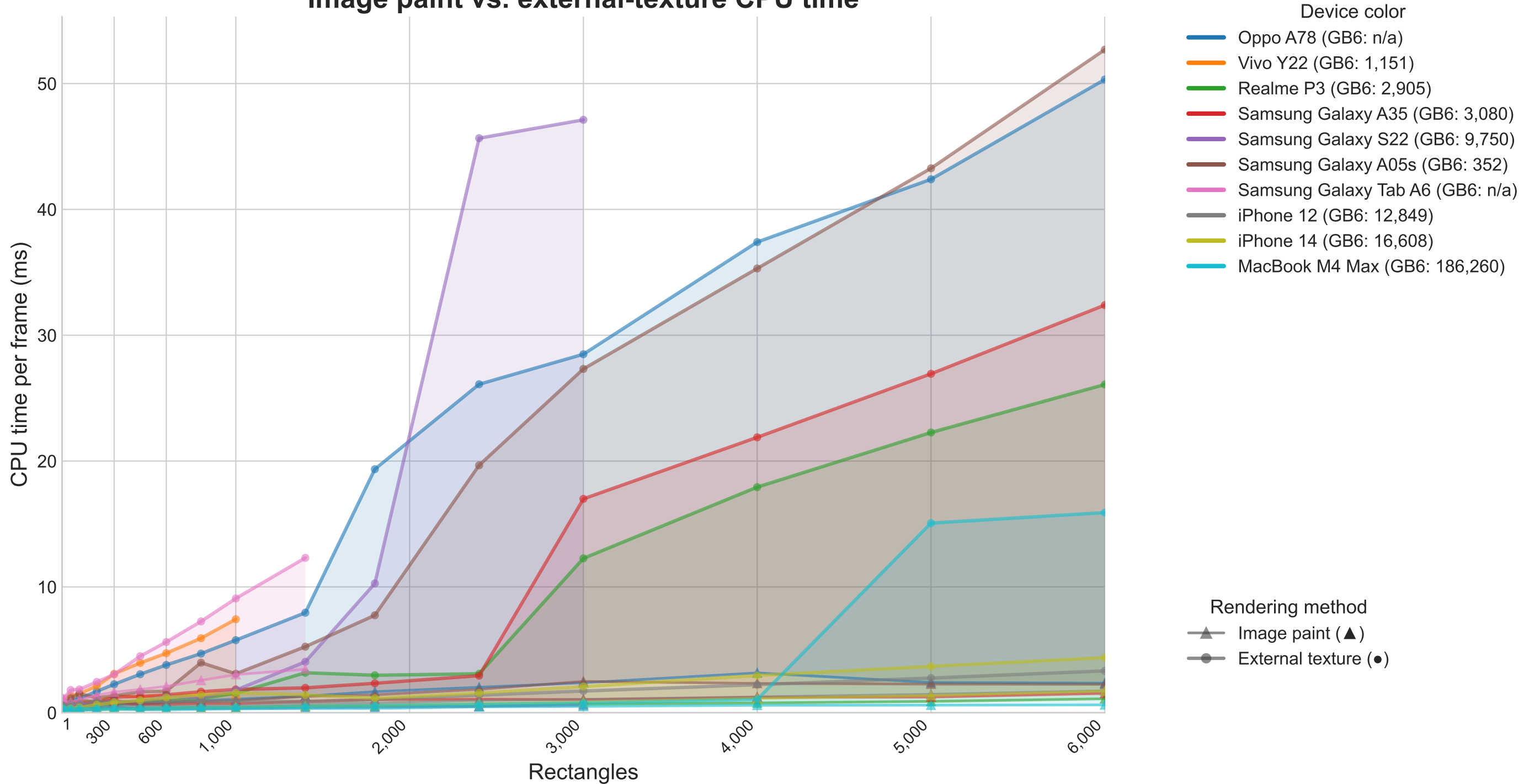
Image paint vs. external-texture CPU time
