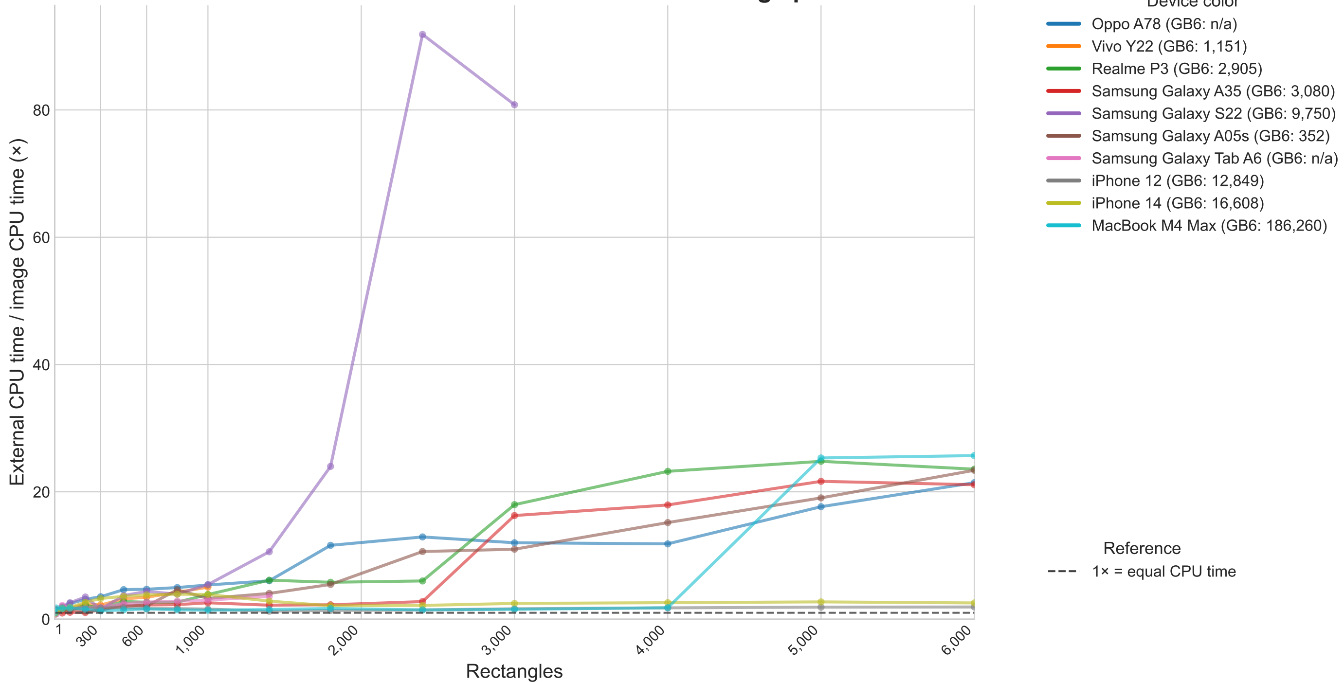
External-texture CPU overhead normalized to image paint
