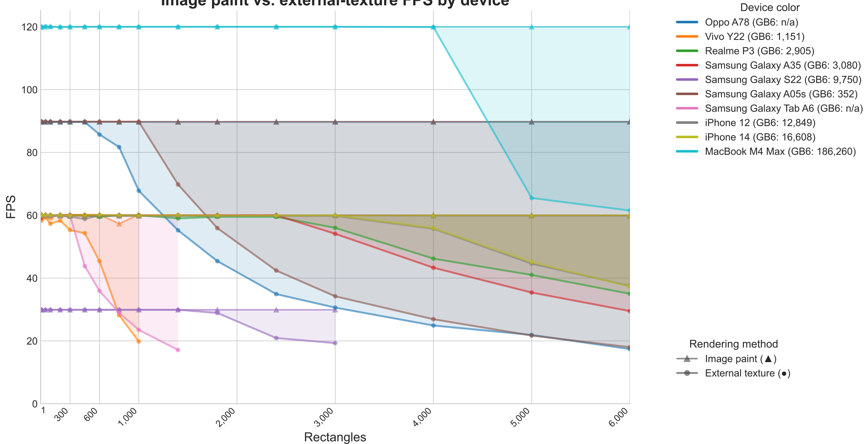
Image paint vs. external-texture FPS by device
